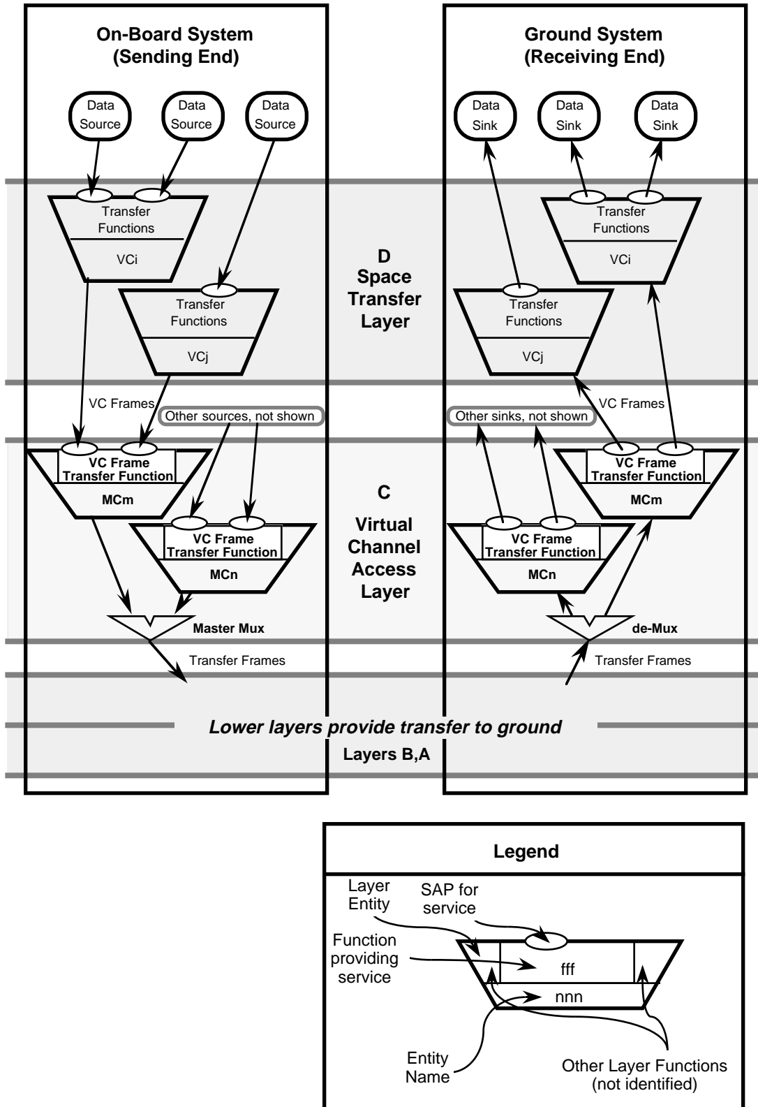
Figure 5-1: VC_Frame Service
