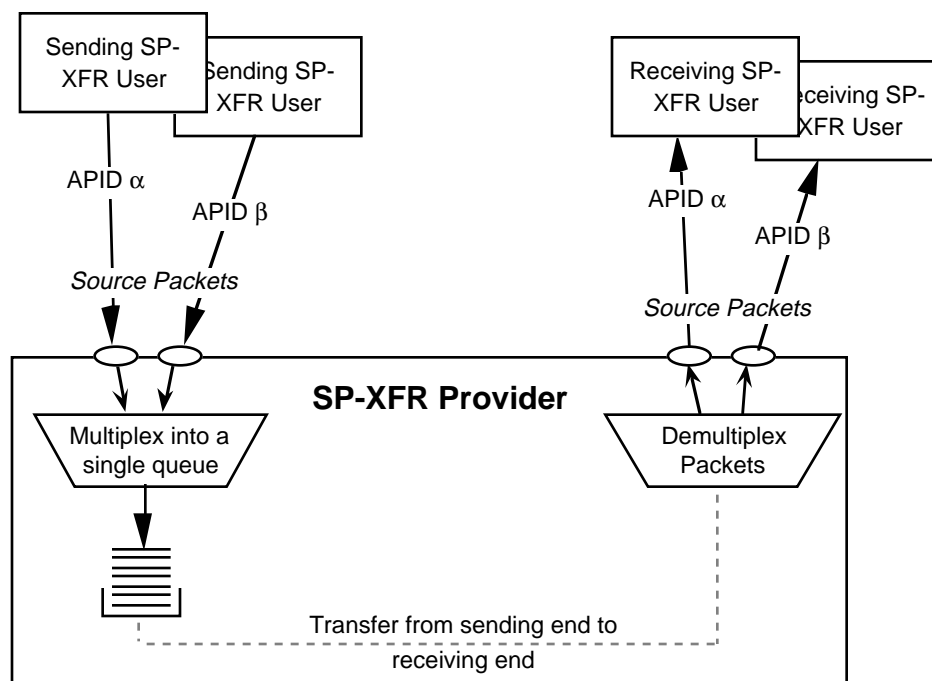
Figure 4-3: Abstract Model of SP-XFR Service
