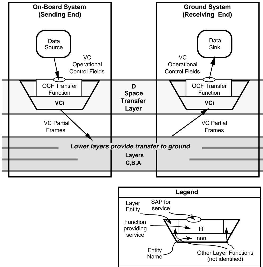
Figure 4-8: VC_OCF Service
