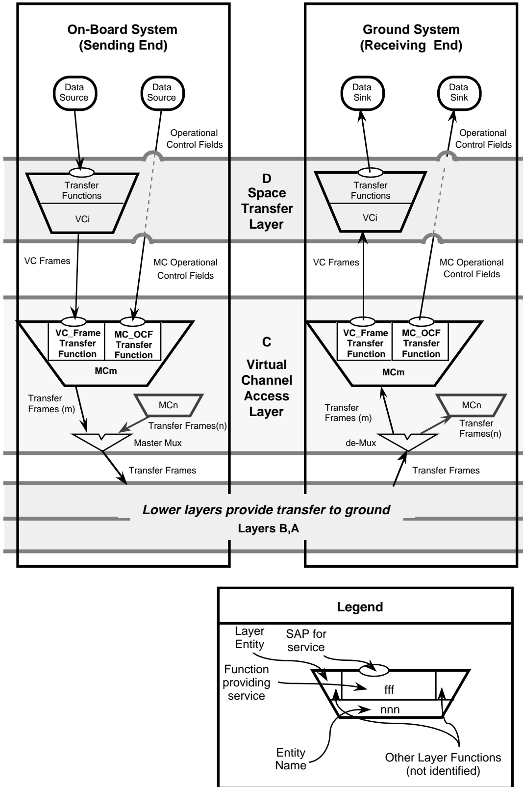
Figure 5-5: MC_OCF Service
