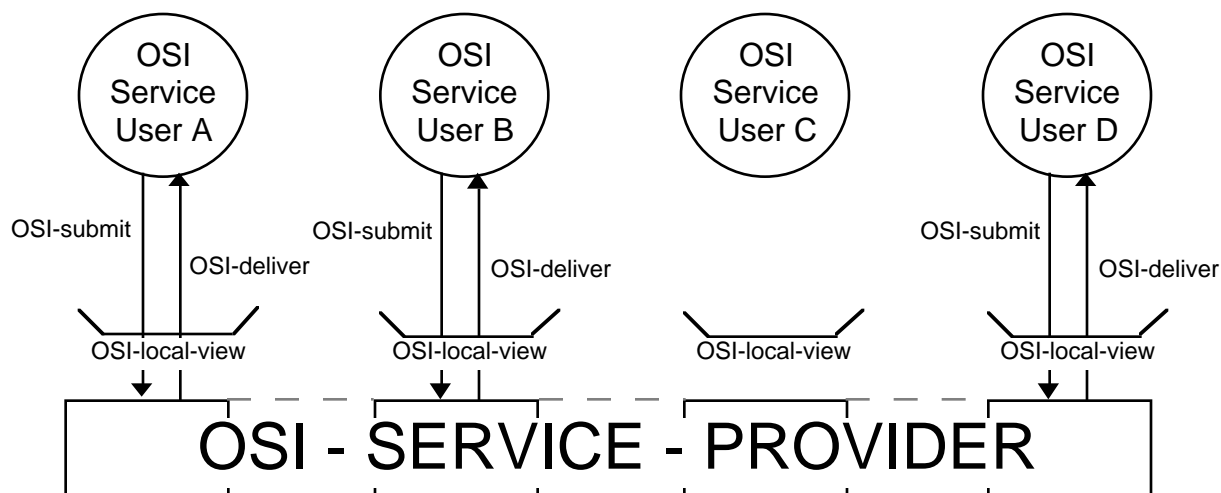
Figure C-1: OSI-Service Model
