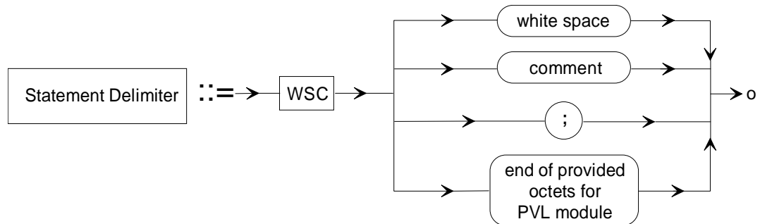
Figure 2-4 Statement Delimiter Syntax Diagram
