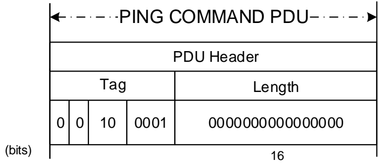
Figure 5-22: Ping Command PDU
