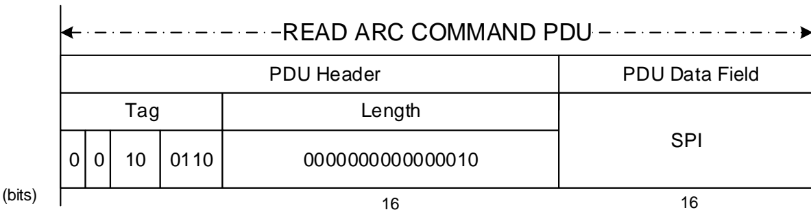
Figure 5-20: Read Sequence Number Command PDU
