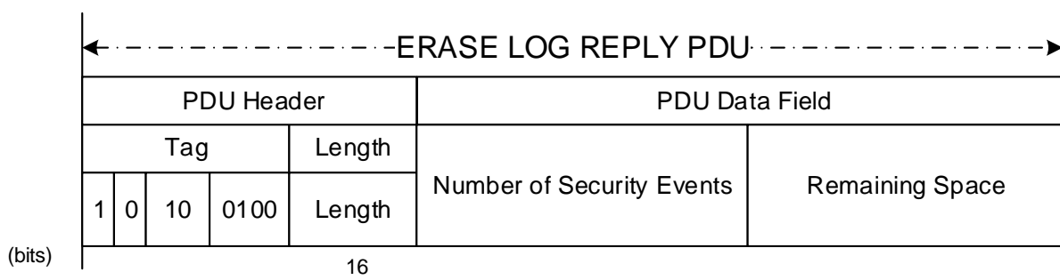
Figure 5-29: Erase Log Reply PDU
