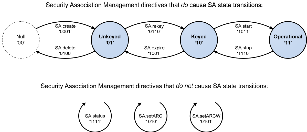
Figure 5-9: SA Management Procedures Overview
