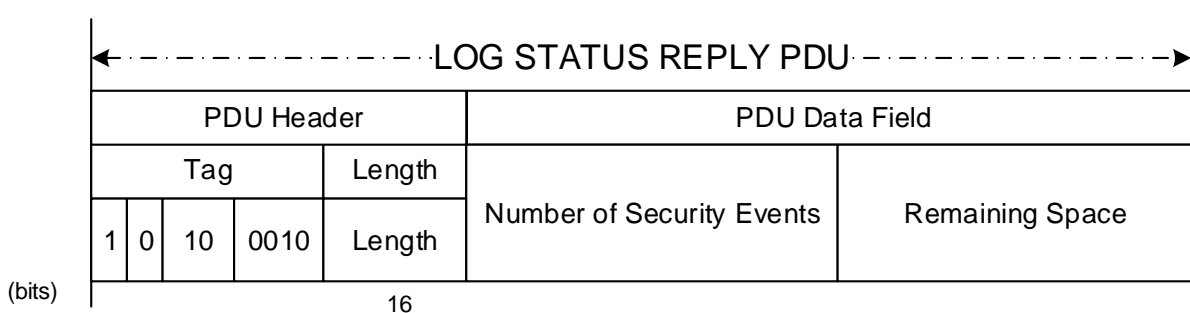
Figure 5-25: Log Status Reply PDU
