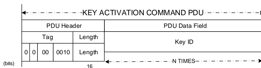
Figure 5-4: Key Activation Command PDU
