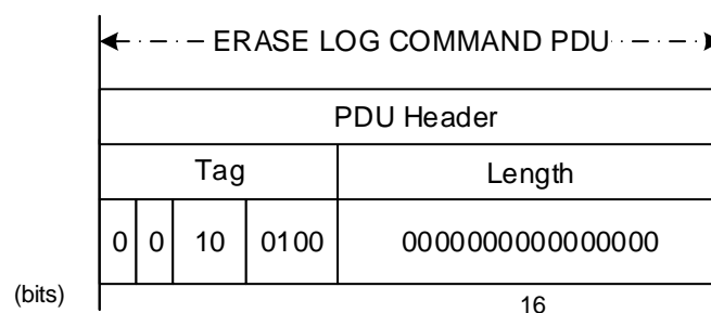
Figure 5-28: Erase Log Command PDU
