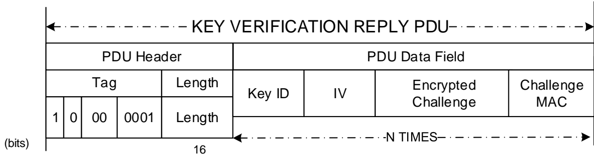
Figure 5-8: Key Verification Reply PDU
