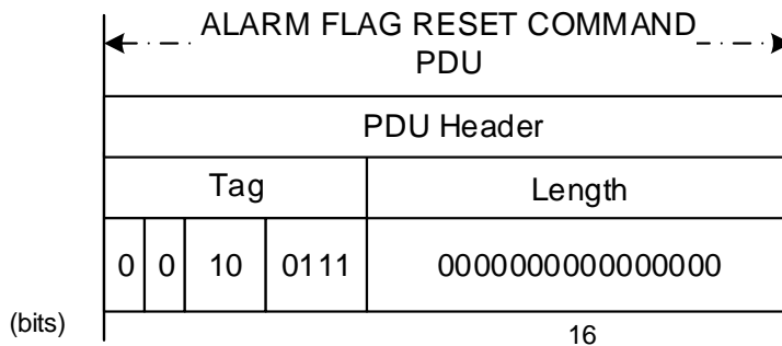
Figure 5-32: Alarm Flag Reset Command PDU
