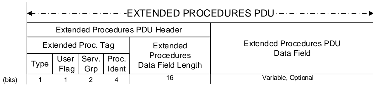
Figure 5-2: Extended Procedures PDU
