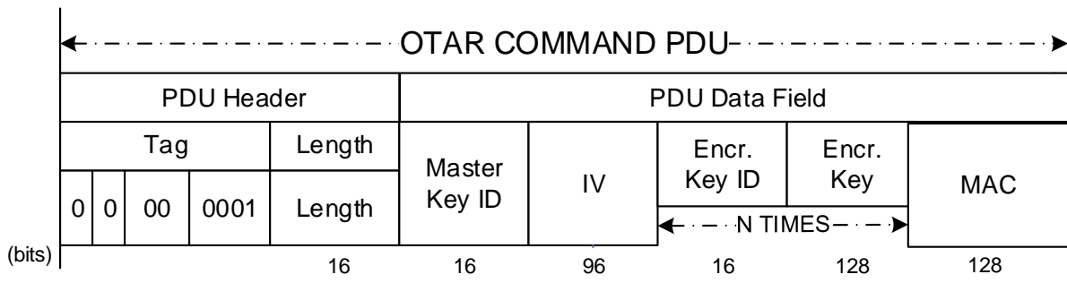
Figure D-1: Baseline Implementation Mode OTAR Command PDU
