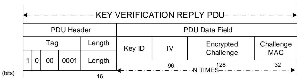
Figure D-5: Baseline Implementation Mode OTAR Reply PDU
