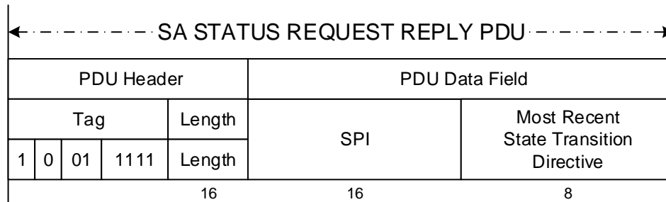
Figure 5-19: SA Status Request Reply PDU
