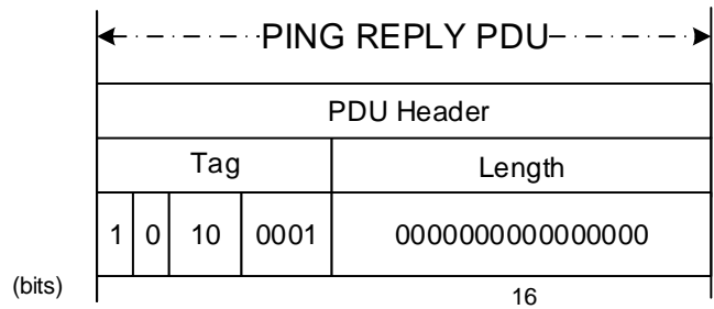
Figure 5-23: Ping Reply PDU
