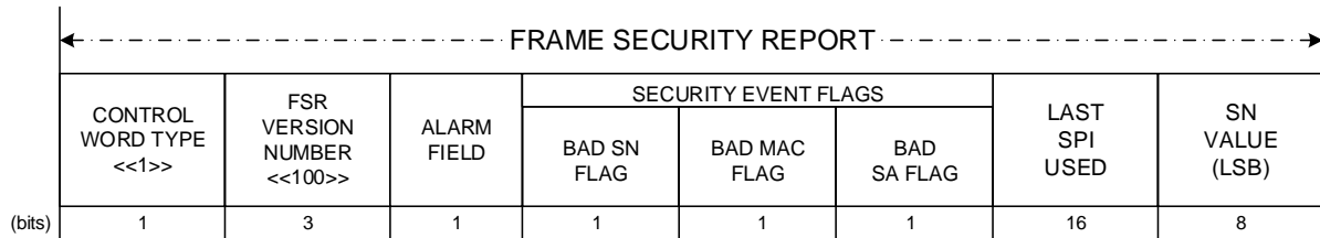
Figure 4-1: Frame Security Report (FSR)
