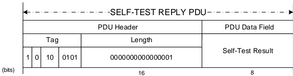
Figure 5-31: Self-Test Reply PDU
