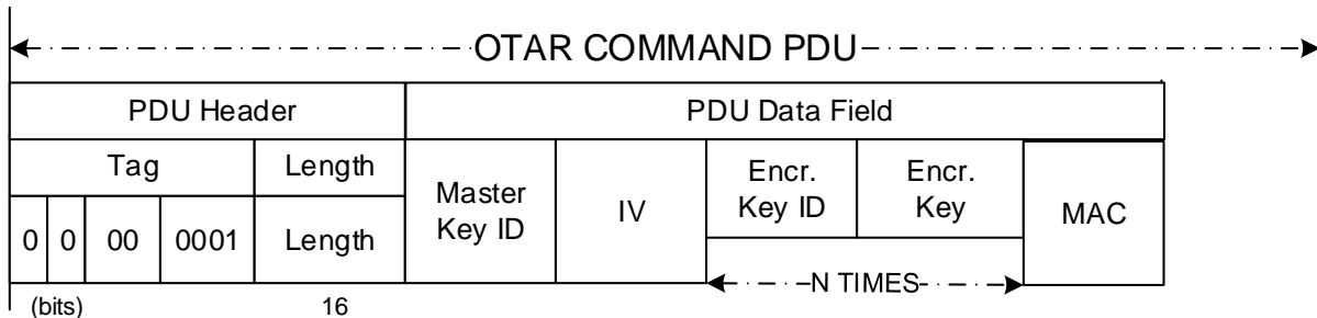
Figure 5-3: OTAR Command PDU
