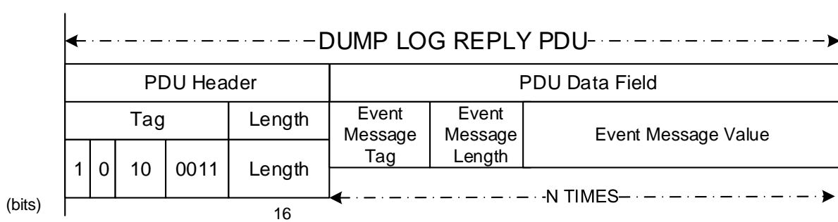
Figure 5-27: Dump Log Reply PDU
