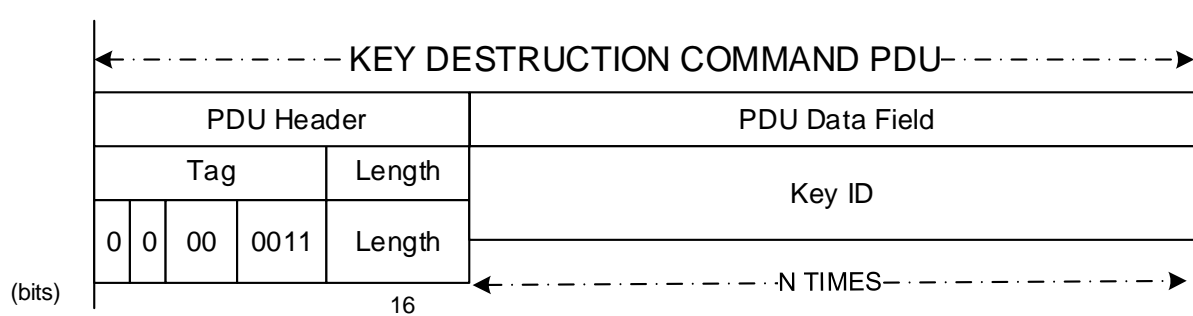
Figure 5-6: Key Destruction Command PDU
