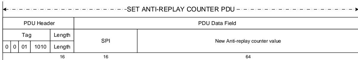
Figure D-10: Set ARC PDU
