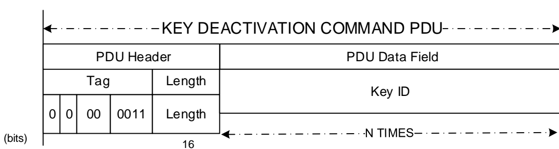
Figure 5-5: Key Deactivation Command PDU
