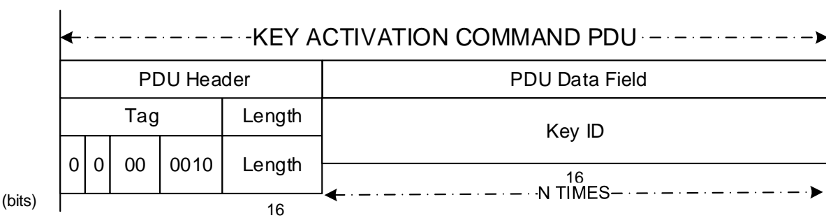
Figure D-2: Baseline Implementation Mode Key Activation Command PDU
