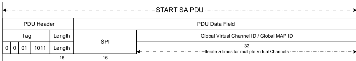
Figure D-6: Baseline Implementation Mode OTAR Reply PDU
