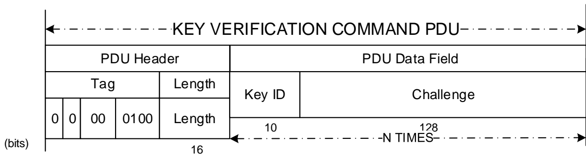
Figure D-4: Baseline Implementation Mode Key Verification Command PDU
