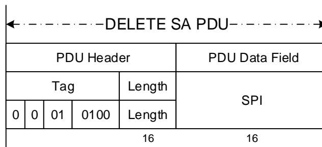
Figure 5-15: Delete SA PDU
