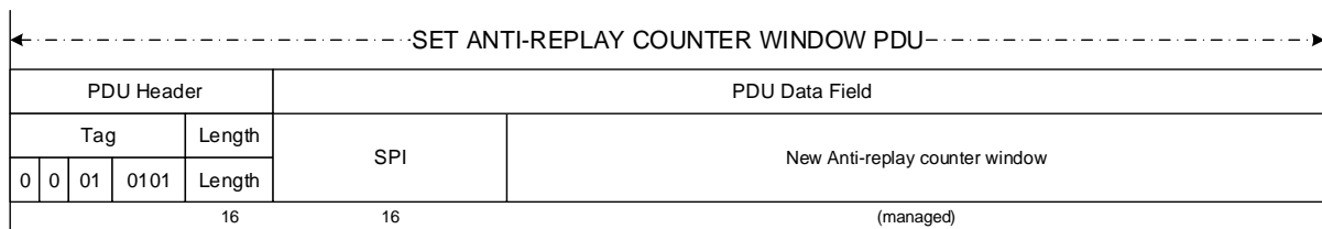
Figure 5-17: Set ARC Window PDU
