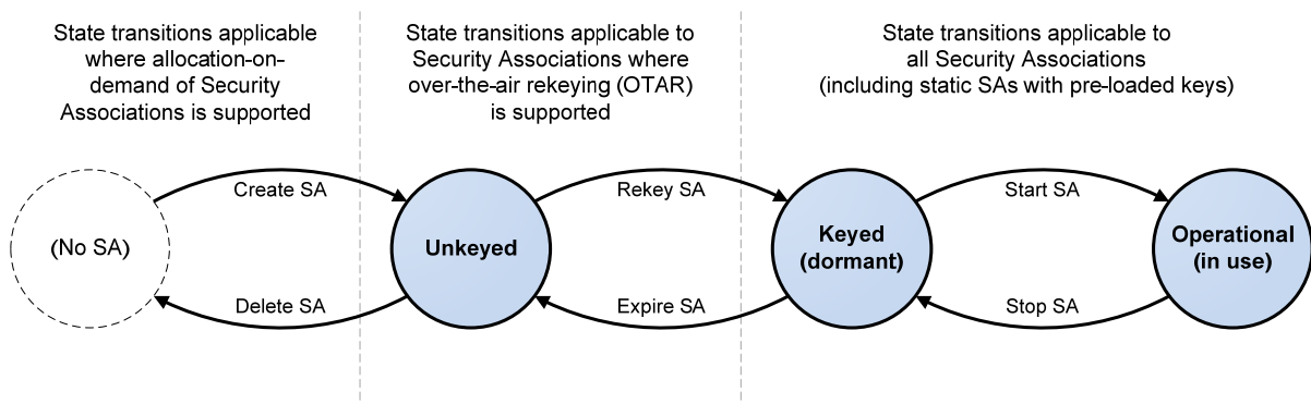
Figure 2-2: Variable State Model for Security Association Management
