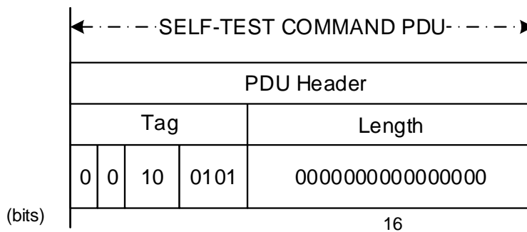
Figure 5-30: Self-Test Command PDU
