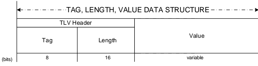
Figure 5-1: TLV Format Specification
