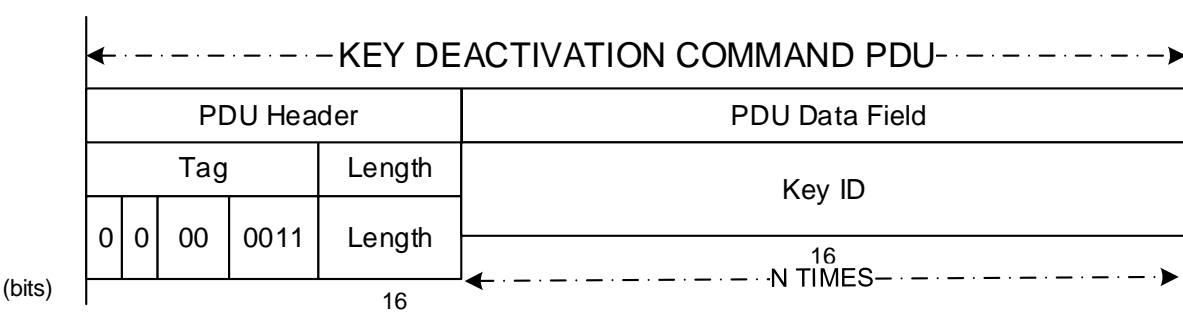
Figure D-3: Baseline Implementation Mode Key Deactivation Command PDU
