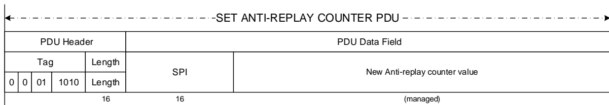
Figure 5-16: Set ARC PDU
