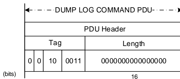
Figure 5-26: Dump Log Command PDU
