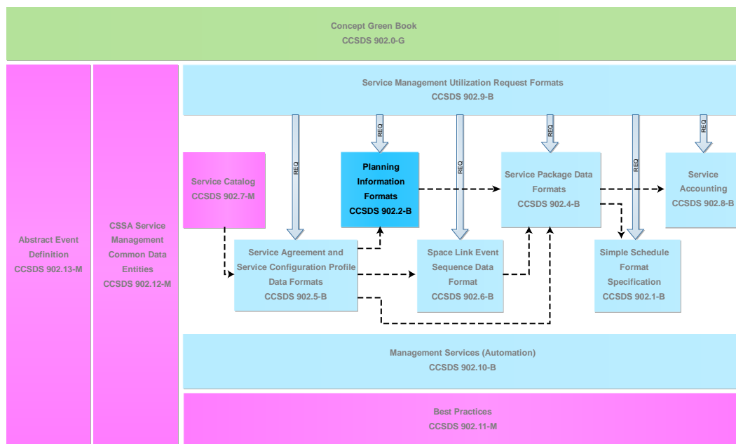
Figure 1-1: Planning Information Formats in the Context of Space Communication Cross Support Service Management
