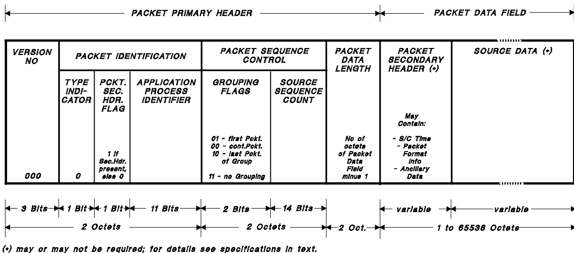
Figure 3-1: Source Packet Format
