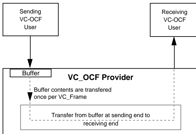
Figure 4-9: Abstract Model of VC_OCF Service
