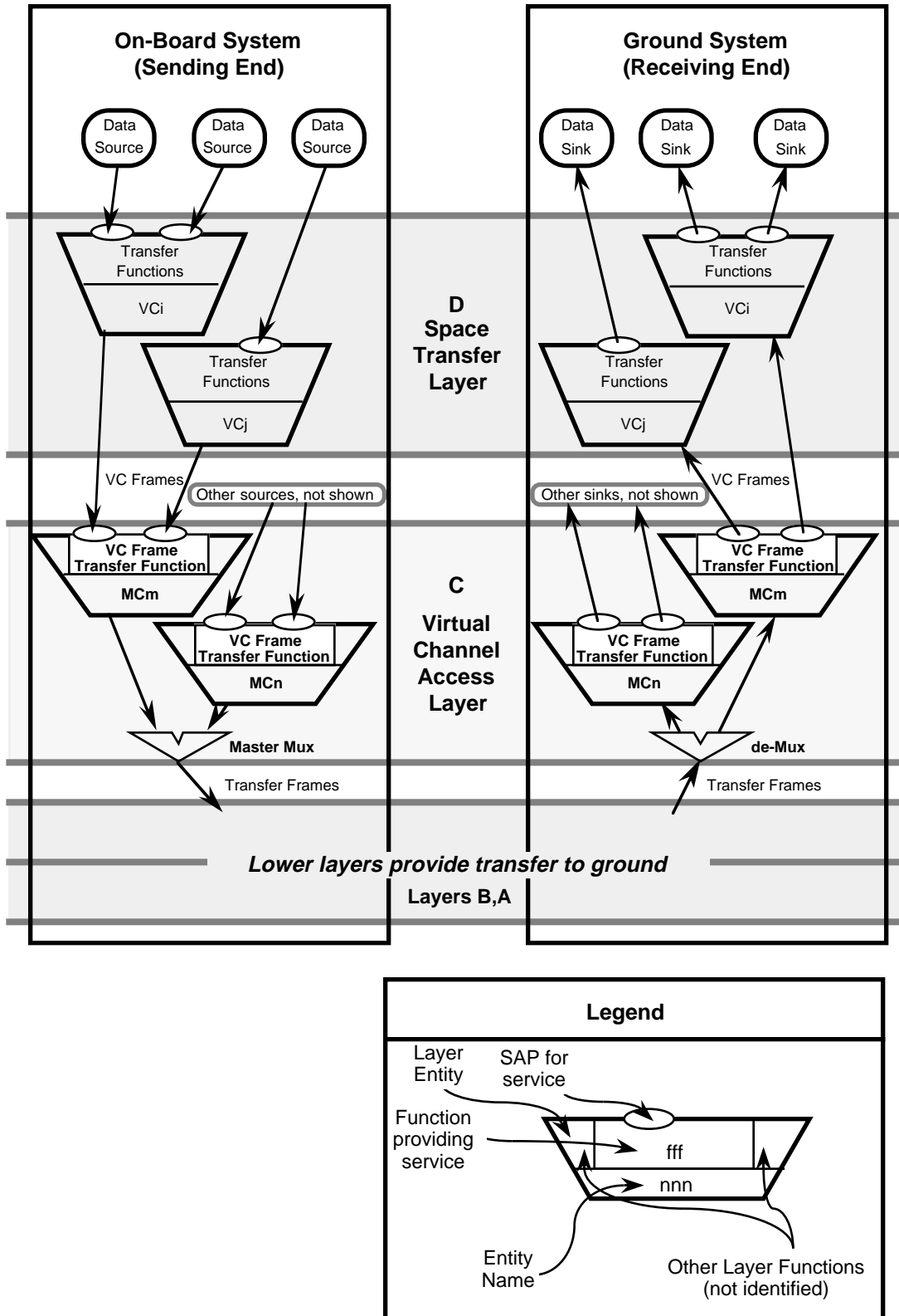
Figure 5-1: VC_Frame Service
