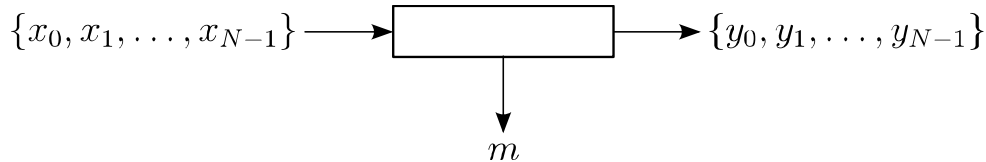
Figure 4-5: Mean-Subtraction Operation
