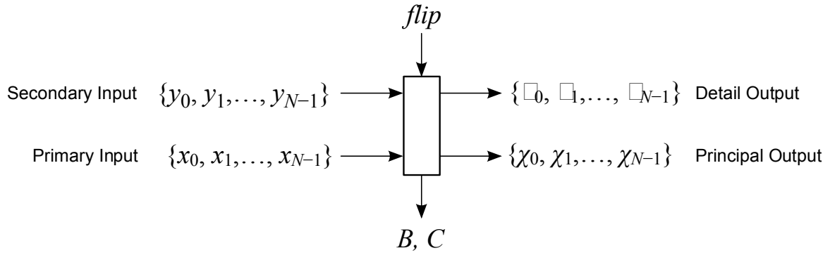
Figure 4-6: The Pairwise Operation
