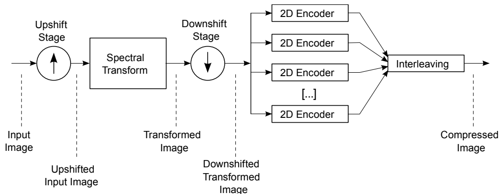
Figure 2-1: Compressor Schematic
