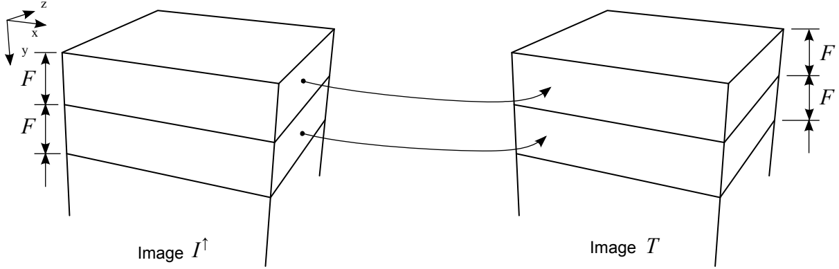
Figure 4-11: Region Partitioning
