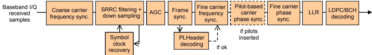
Figure 3-3: Functional Diagram of a Typical DVB-S2 Receiver
