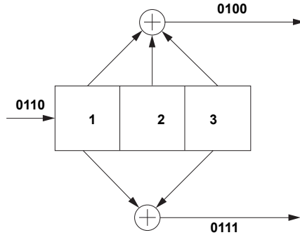
Figure 4-4: (3,1/2) Convolutional Encoder
