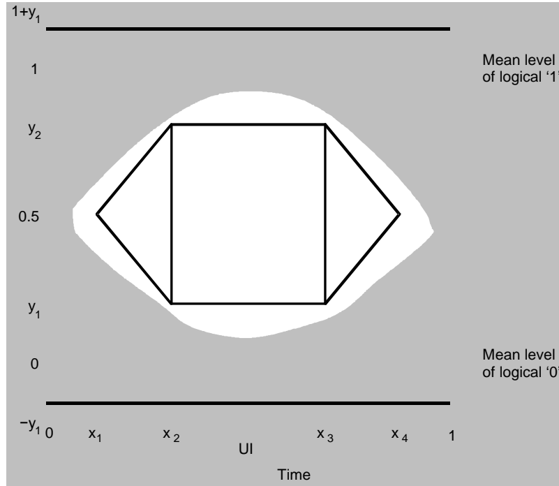
Figure 3-11: Transmit Eye Pattern
