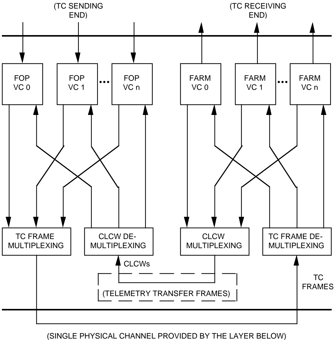
Figure 4-1: Orientation of the Transfer Layer
