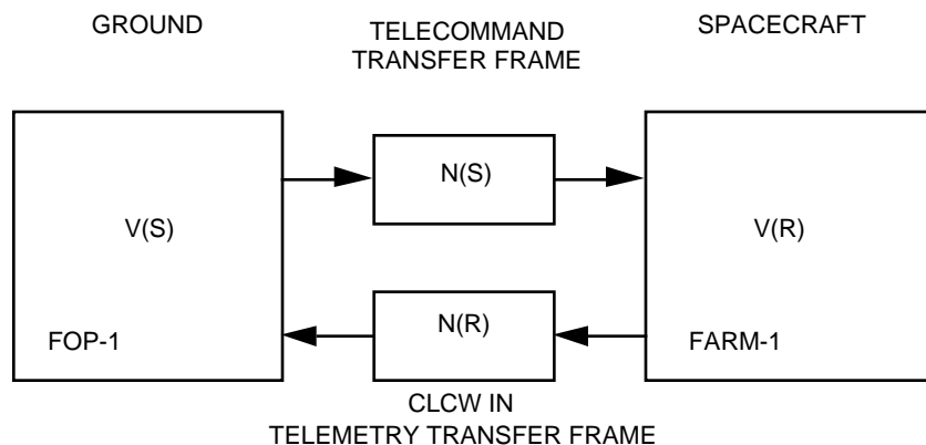
Figure 2-1: COP-1 Variables, Frame and Report Values
