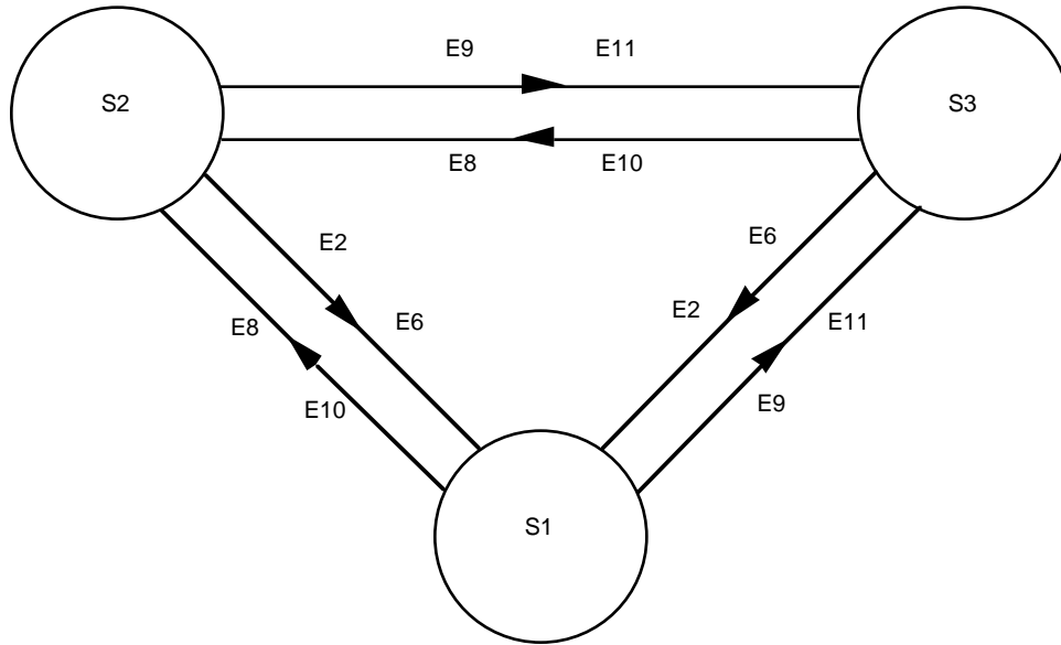
Figure 2-3: FOP-1 State Transitions: Main Protocol
