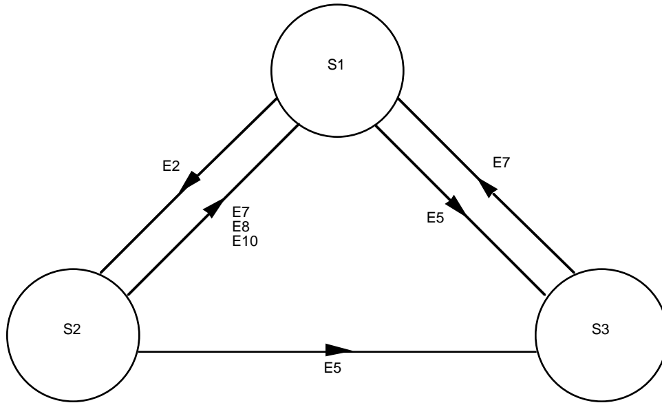
Figure 2-6: FARM-1 State Transitions
