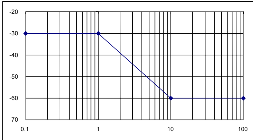
Figure 3-2: Discrete Lines Template for the Transmitter (Normalized Power in dBc vs. Normalized Frequency: f/A )
