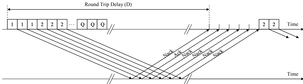
Figure G-2: Go-Back-N Scheme with Multiple Copies (MGBN)
