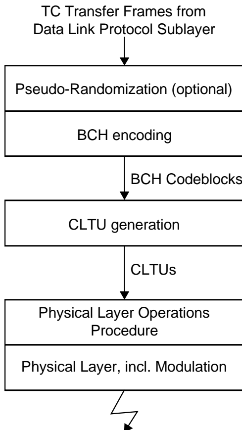
Figure 2-2: Procedures at the Sending End
