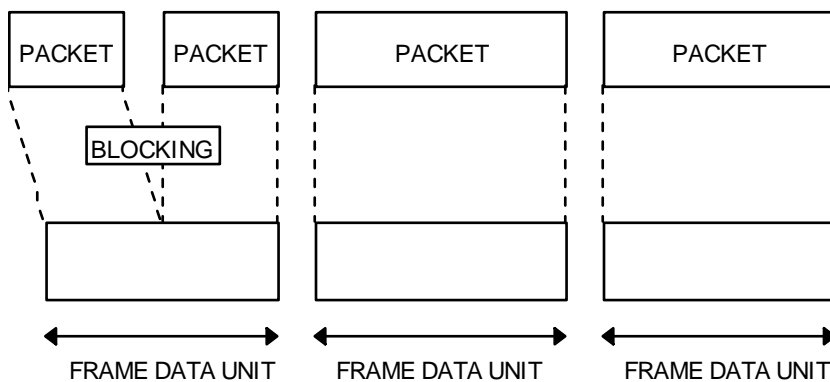
Figure 4-12: Example of VC Packet Processing Procedures
