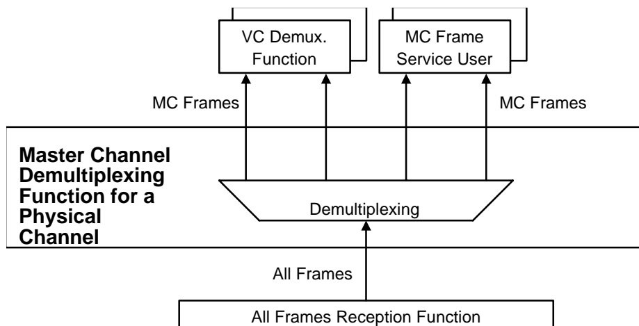
Figure 4-24: Abstract Model of Master Channel Demultiplexing Function
