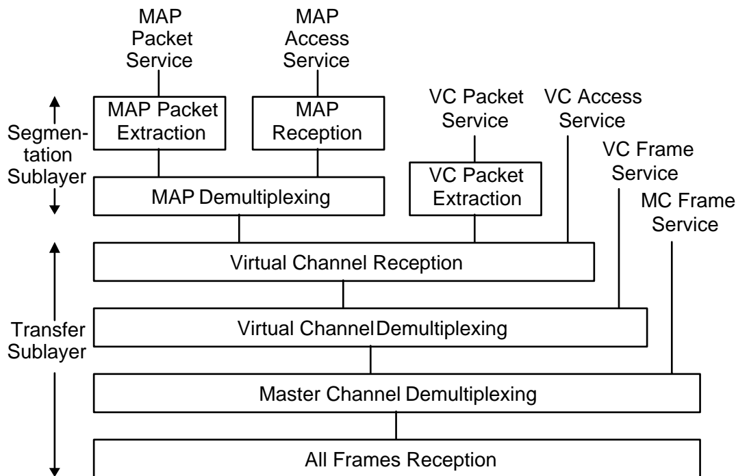
Figure 4-17: Internal Organization of Protocol Entity (Receiving End)
