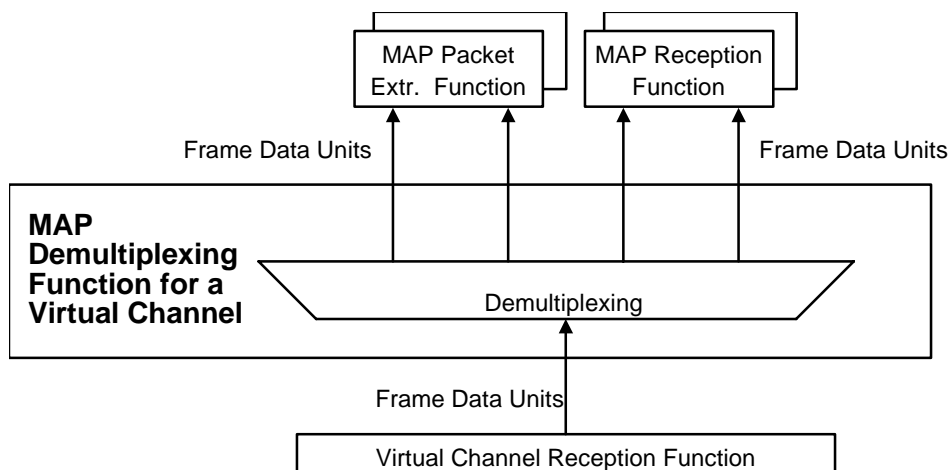
Figure 4-20: Abstract Model of MAP Demultiplexing Function
