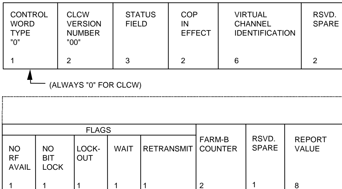
Figure 4-4: Communications Link Control Word
