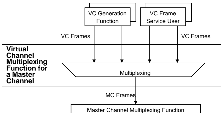
Figure 4-14: Abstract Model of Virtual Channel Multiplexing Function
