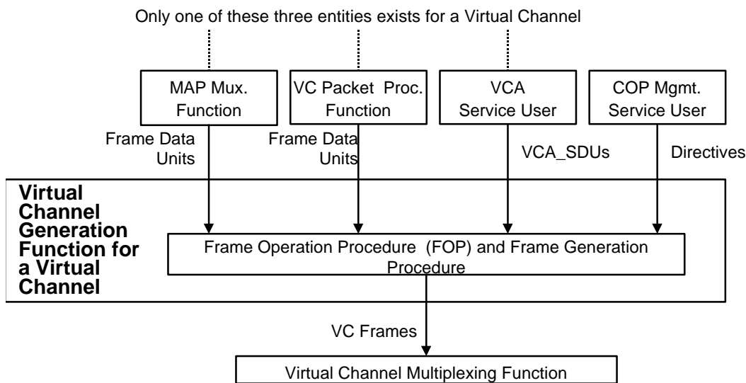
Figure 4-13: Abstract Model of Virtual Channel Generation Function
