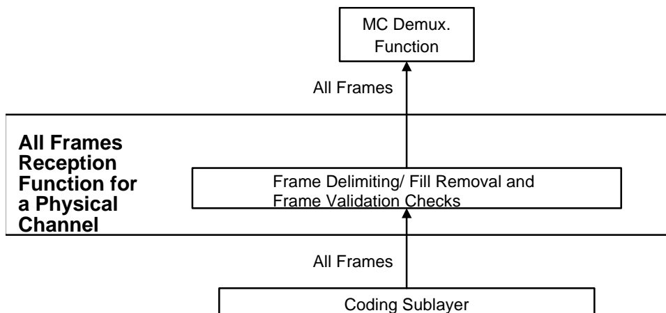
Figure 4-25: Abstract Model of All Frames Reception Function
