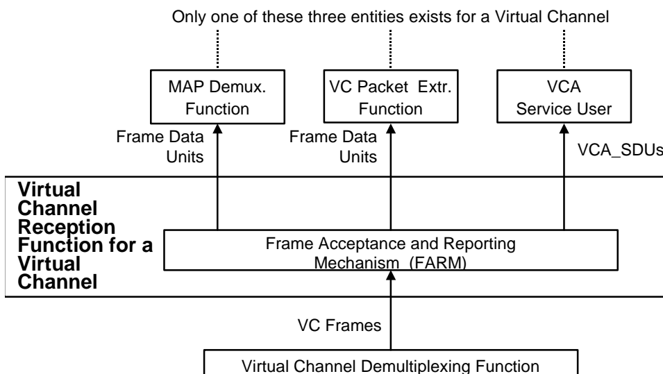
Figure 4-22: Abstract Model of Virtual Channel Reception Function
