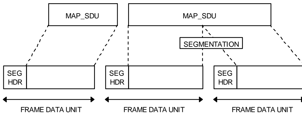
Figure 4-9: Example of MAP Generation Procedures
