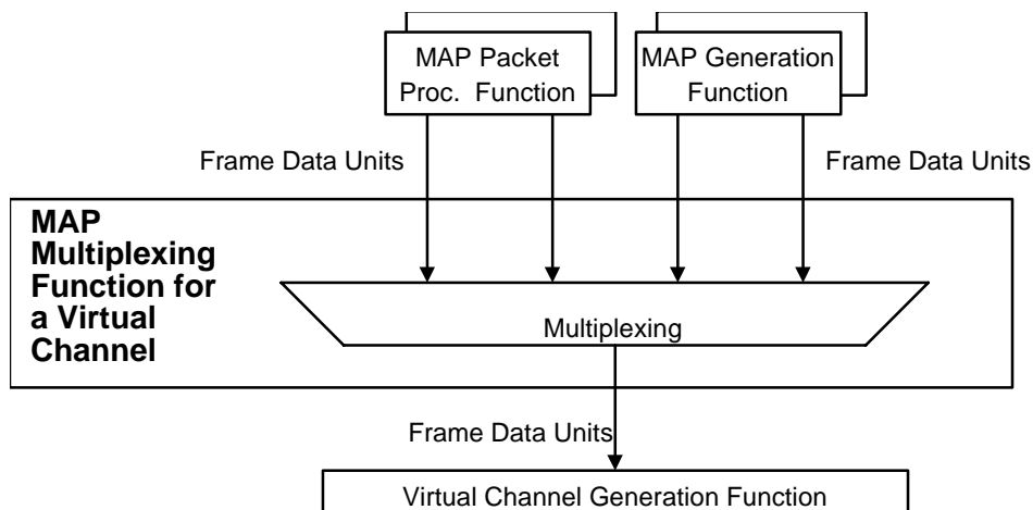
Figure 4-10: Abstract Model of MAP Multiplexing Function
