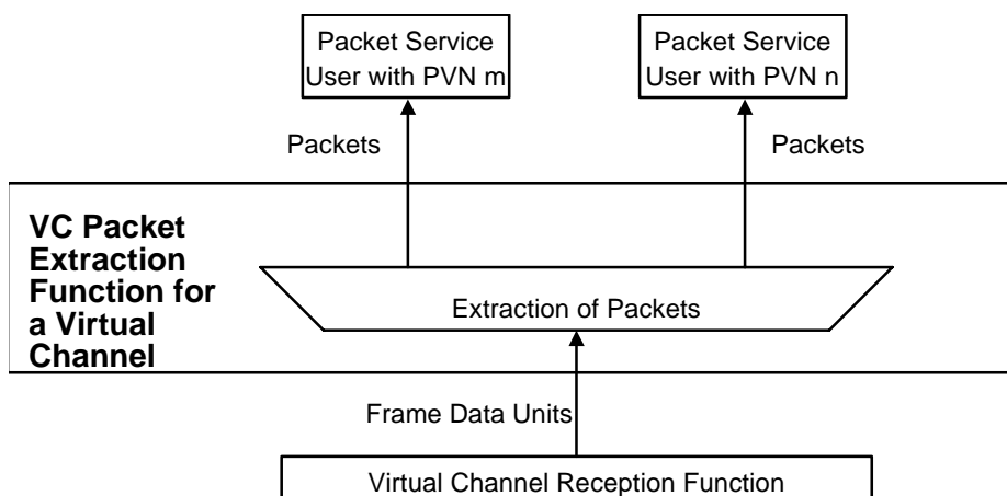
Figure 4-21: Abstract Model of VC Packet Extraction Function
