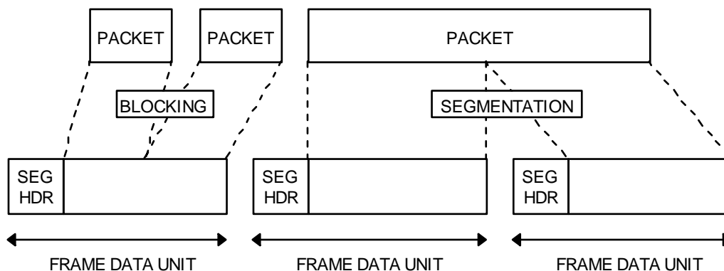
Figure 4-7: Example of MAP Packet Processing Procedures
