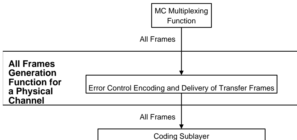
Figure 4-16: Abstract Model of All Frames Generation Function
