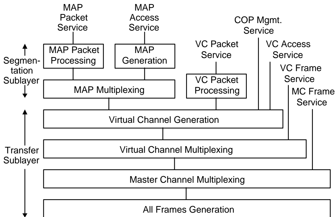
Figure 4-5: Internal Organization of Protocol Entity (Sending End)
