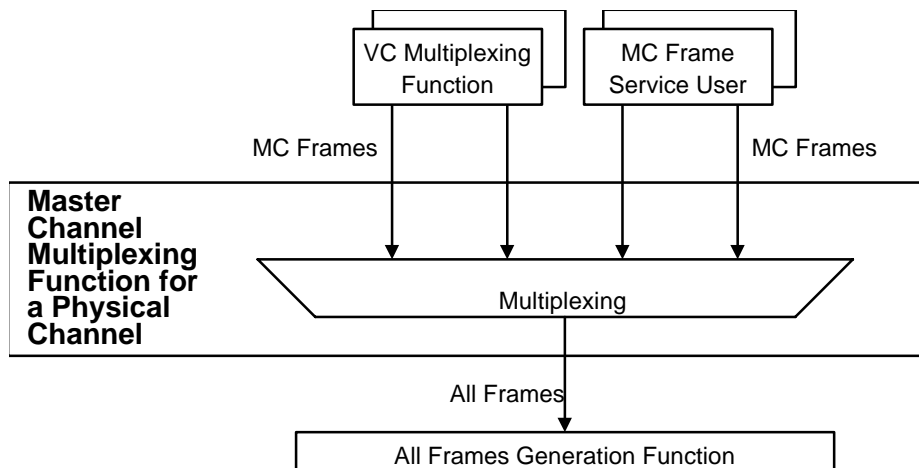
Figure 4-15: Abstract Model of Master Channel Multiplexing Function
