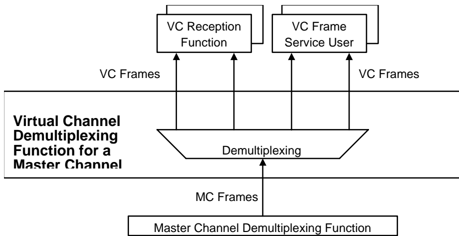
Figure 4-23: Abstract Model of Virtual Channel Demultiplexing Function
