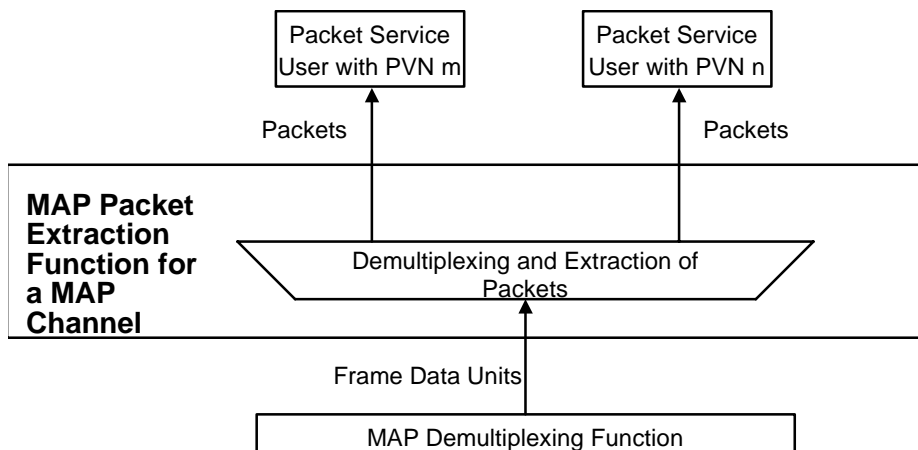
Figure 4-18: Abstract Model of MAP Packet Extraction Function
