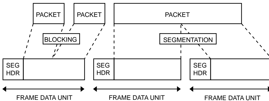
Figure 4-9: Example of MAP Packet Processing Procedures
