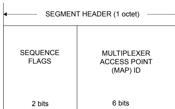
Figure 4-3: Segment Header
