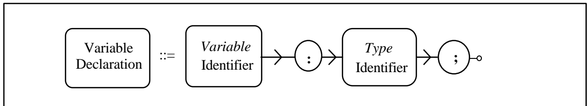
Figure 3-31: Variable Declaration Diagram
