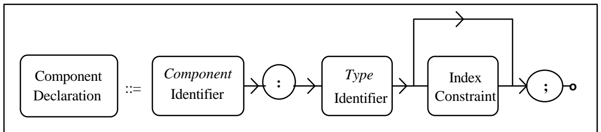
Figure 3-21: Component Declaration Diagram
