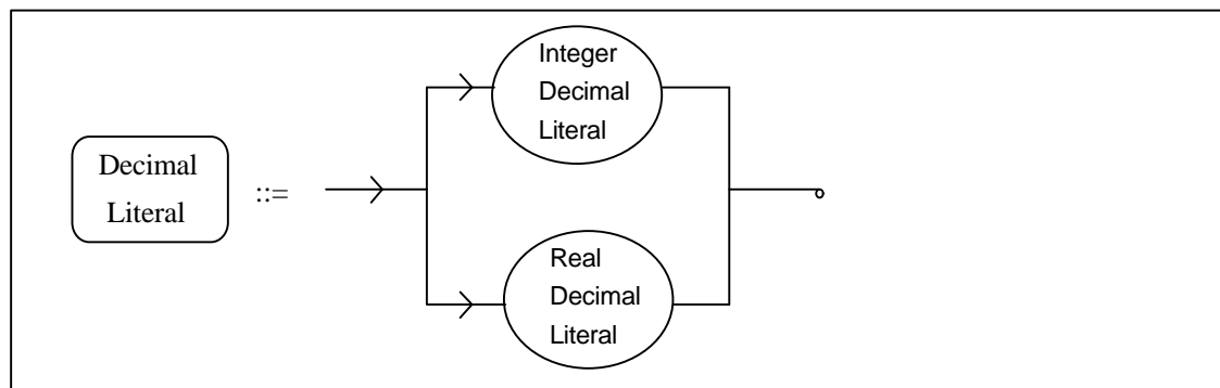
Figure 3-2: Decimal Literal Definition Diagram
