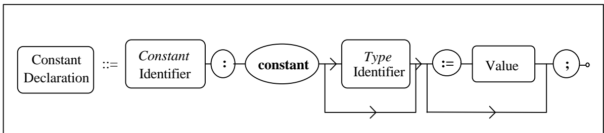
Figure 3-32: Constant Declaration Diagram
