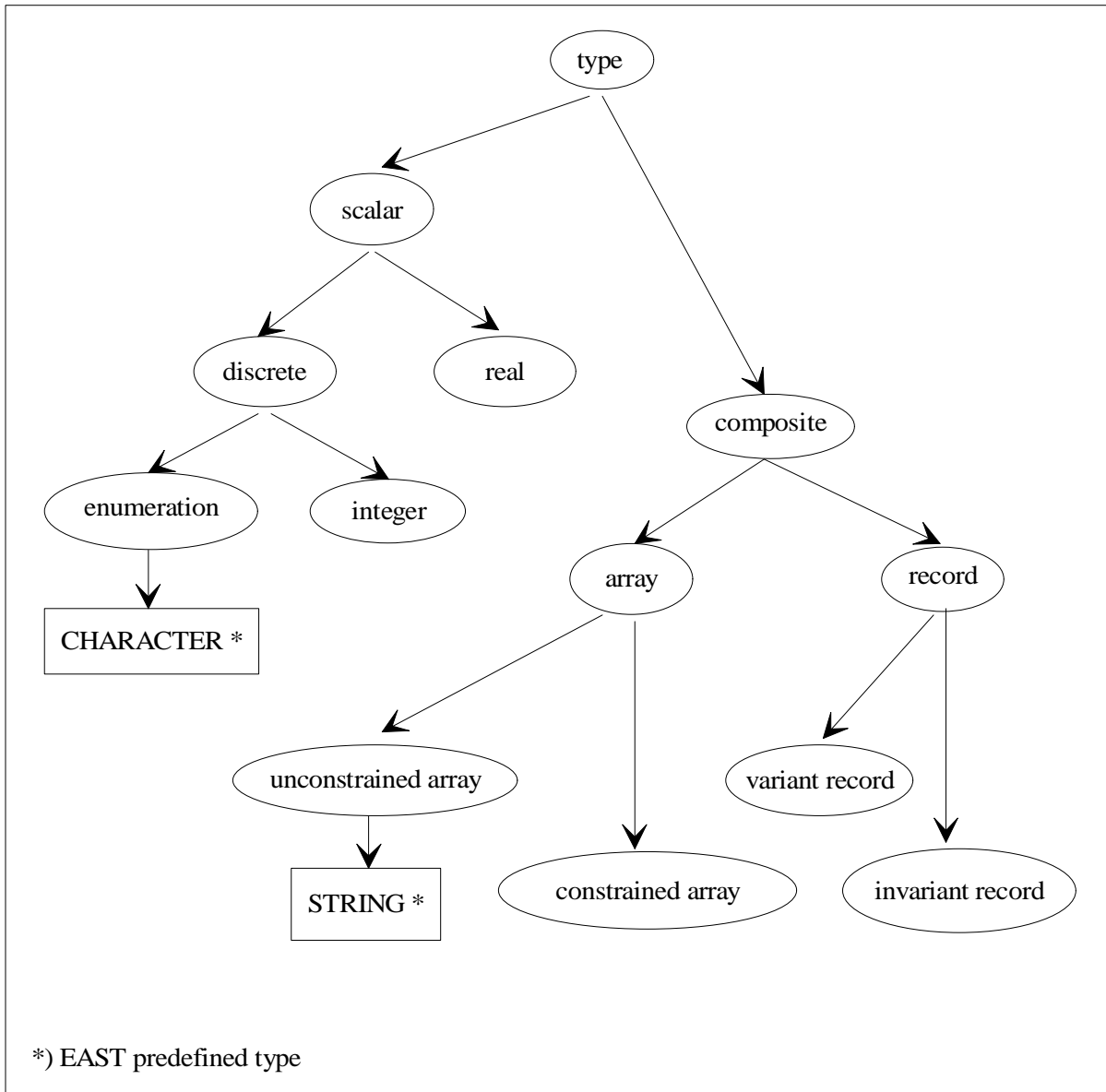
Figure 3-26: Type Summary
