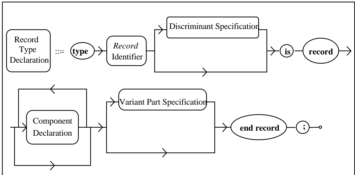
Figure 3-20: Record Type Specification Diagram
