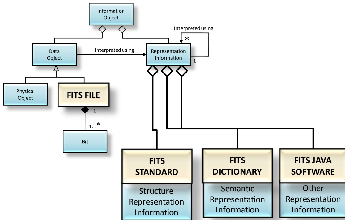
Figure 4-13: Example of a Simplified RIN for a FITS File
