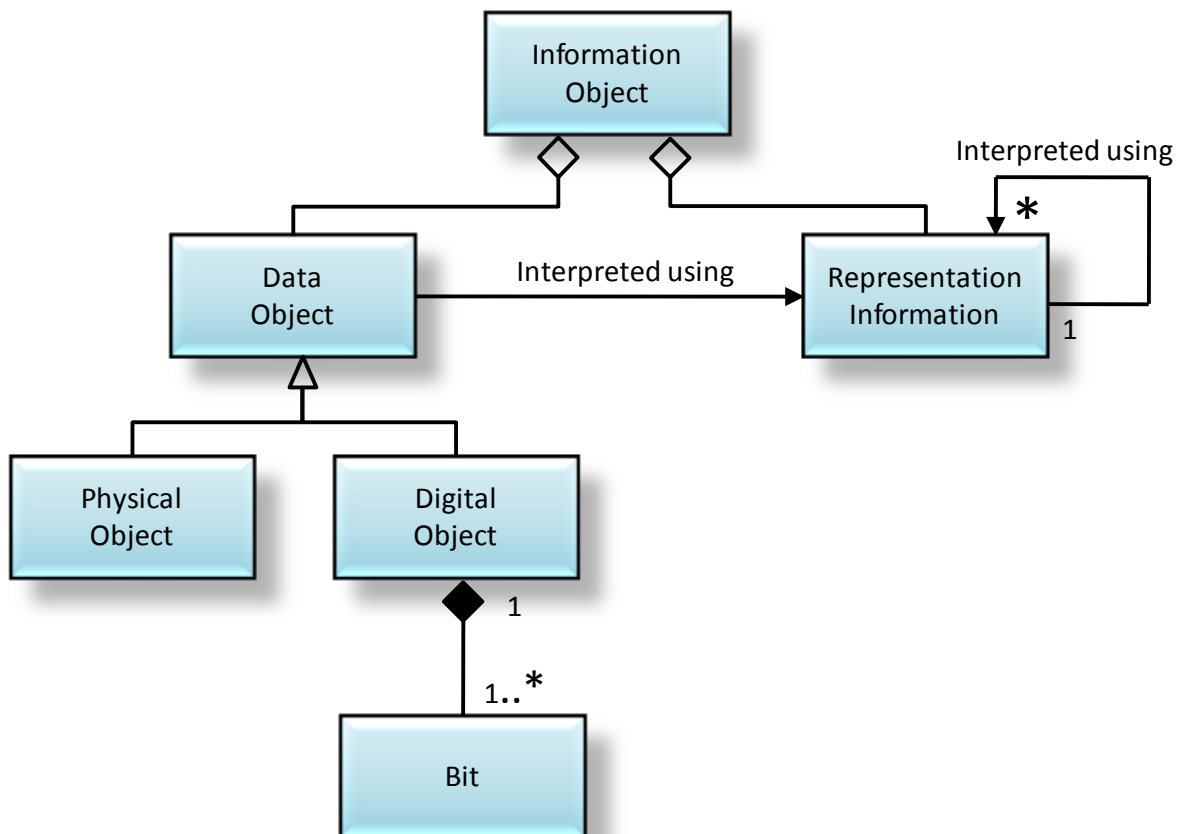
Figure 4-10: Information Object
