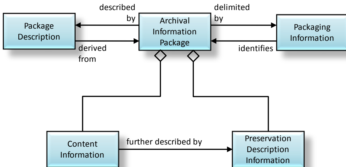
Figure 4-18: Archival Information Package (AIP) and Its Associated Package Description and Packaging Information
