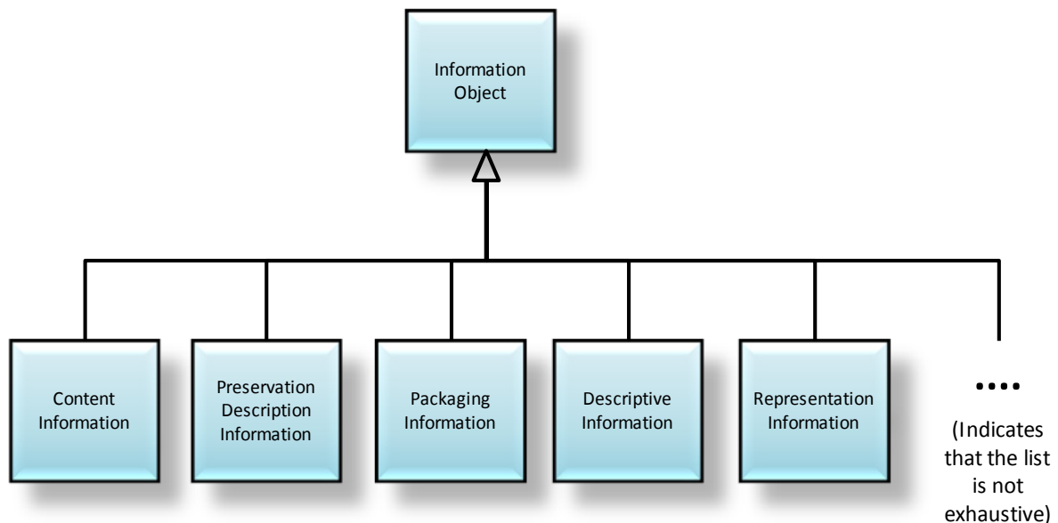
Figure 4-14: Information Object Taxonomy
