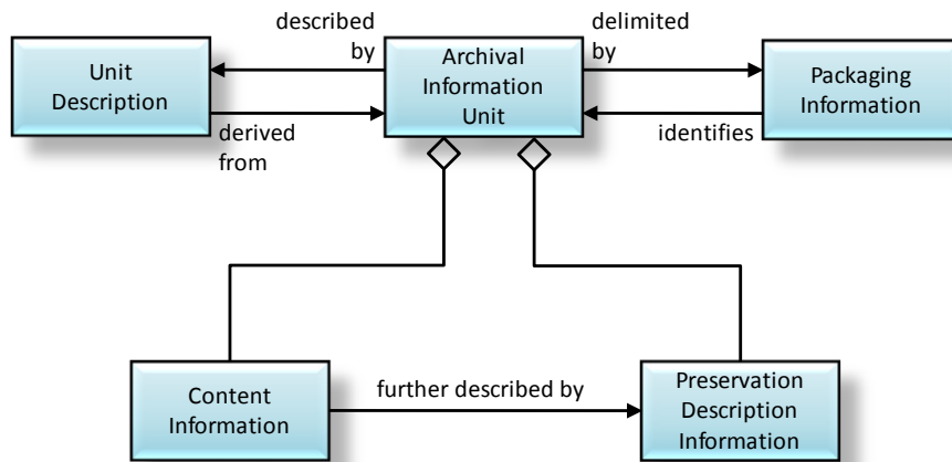
Figure 4-24: Archival Information Unit (AIU) and Its Associated Unit Description and Packaging Information
