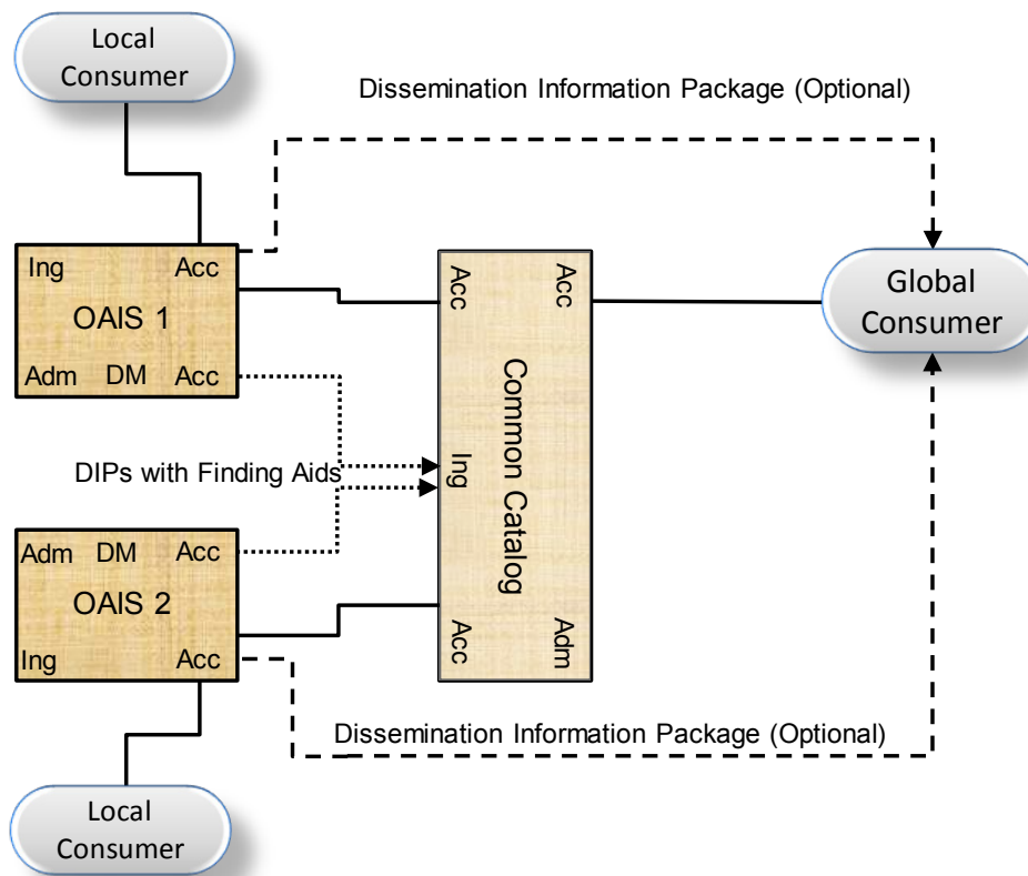
Figure 6-3: An OAIS Federation Employing a Common Catalog
