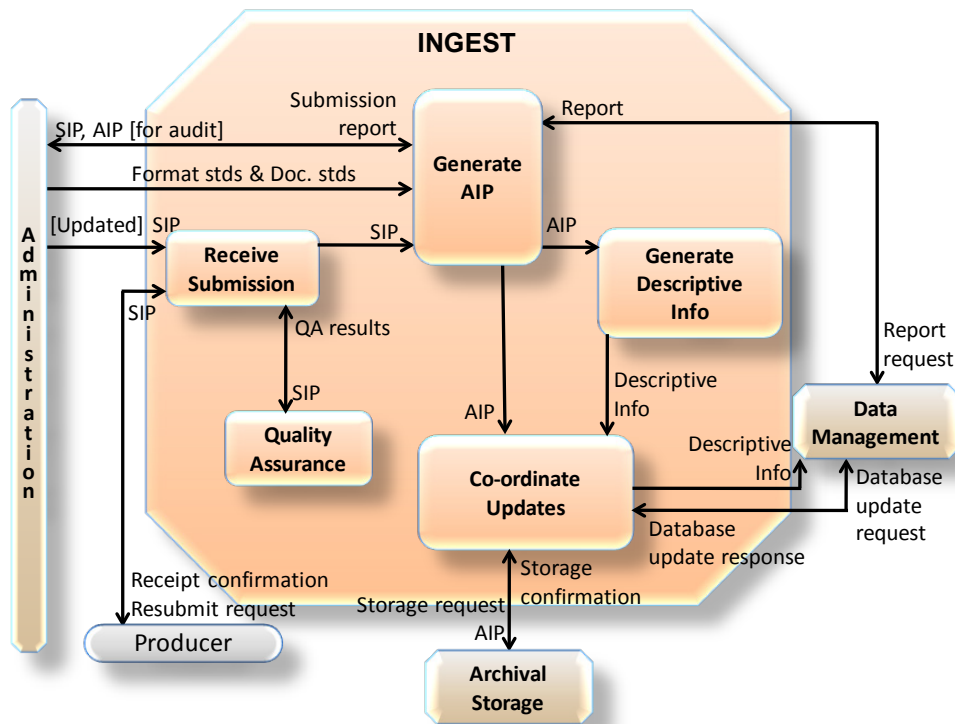
Figure 4-2: Functions of the Ingest Functional Entity
