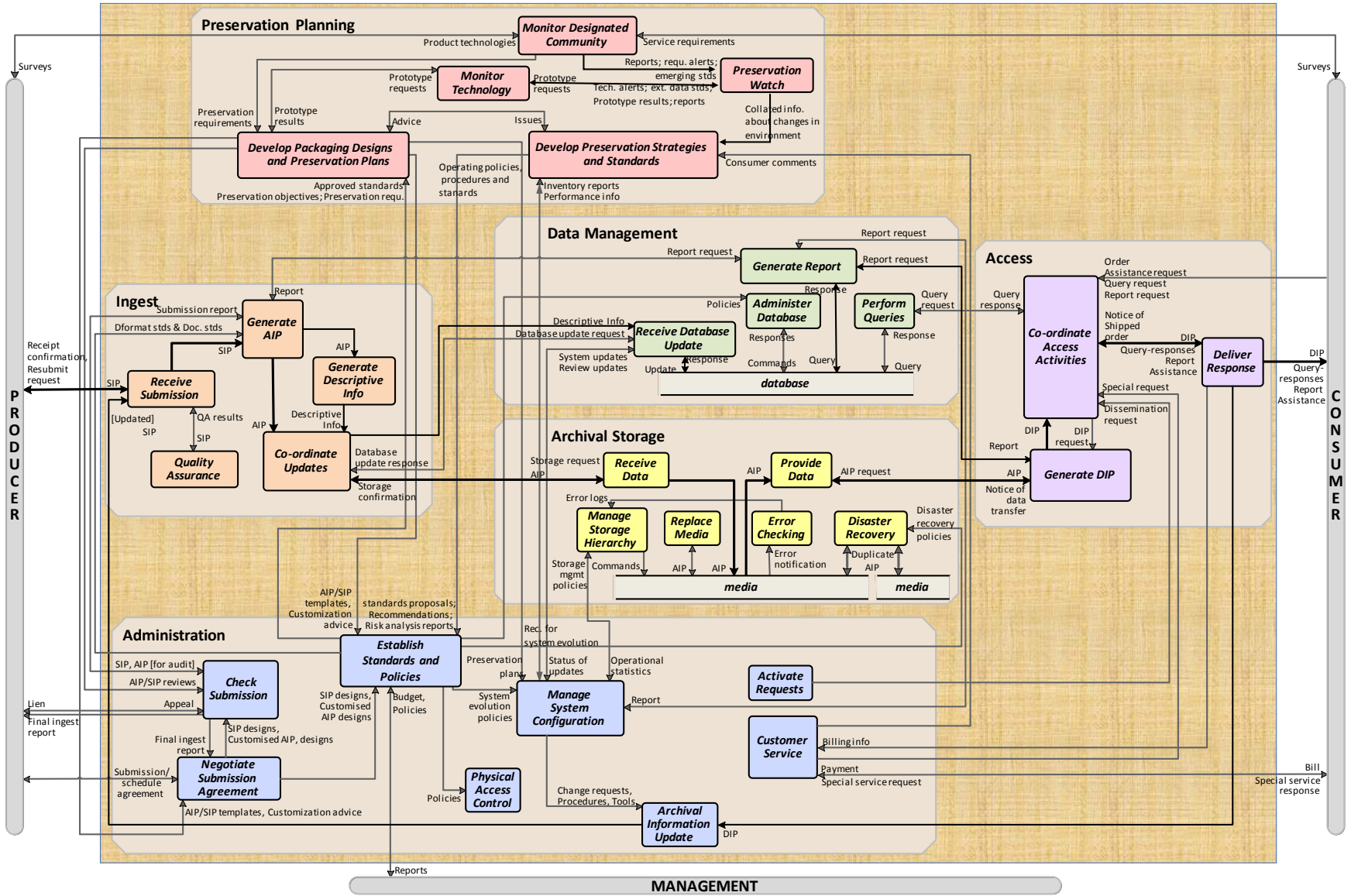
Figure A-1: Composite of Functional Entities
