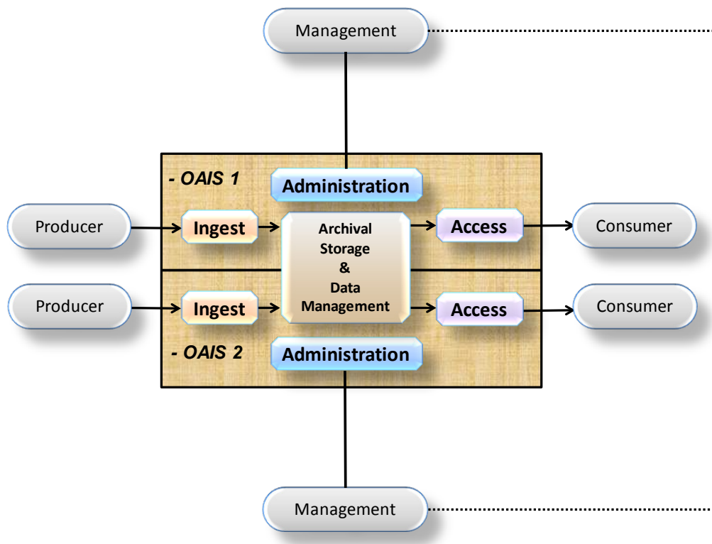
Figure 6-4: Archives with Shared Storage
