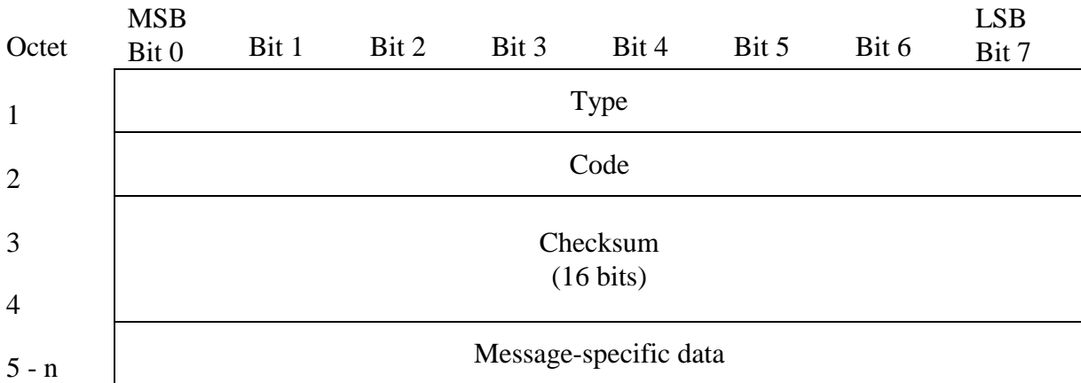
Figure 3-4: SCPS Control Message Protocol Header Format
