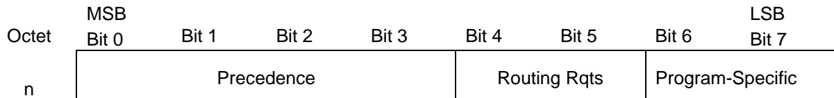
Figure 3-3: SCPS-NP Header - Basic Quality of Service Field
