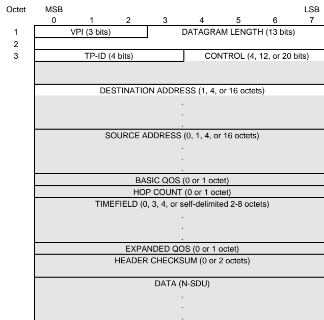
Figure 3-1: SCPS-NP Datagram
