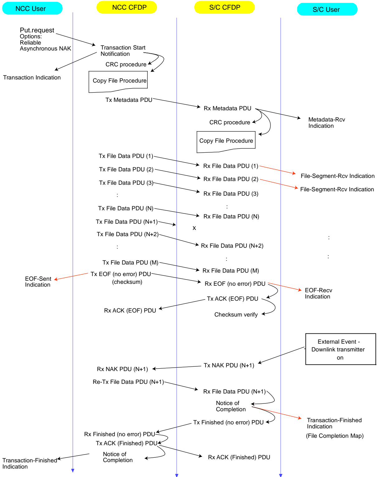
Figure 3-5: Reliable Upload
