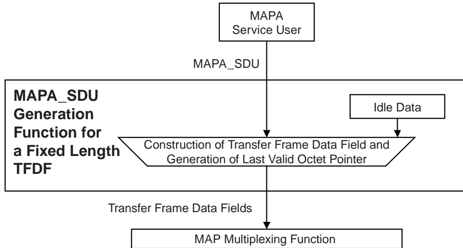
Figure 4-9: Abstract Model of MAPA_SDU Generation Function for Fixed-Length TFDFs
