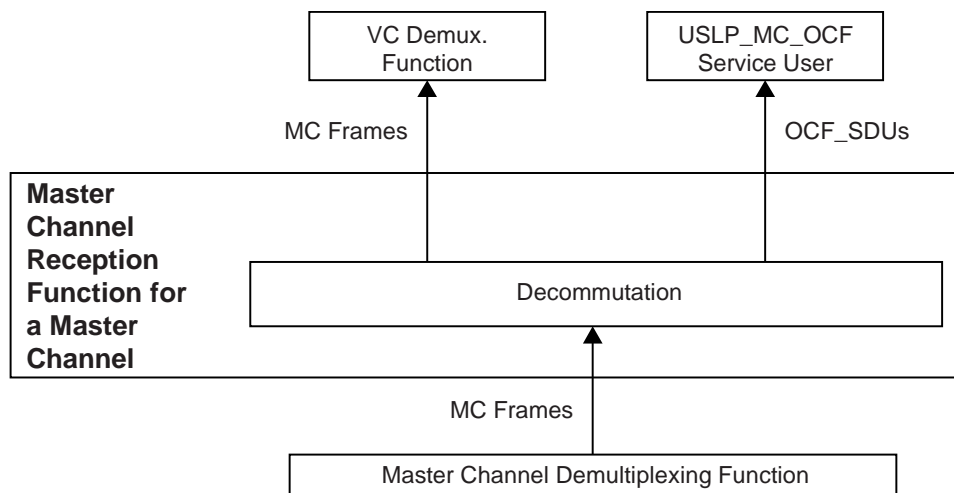
Figure 4-27: Abstract Model of Master Channel Reception Function
