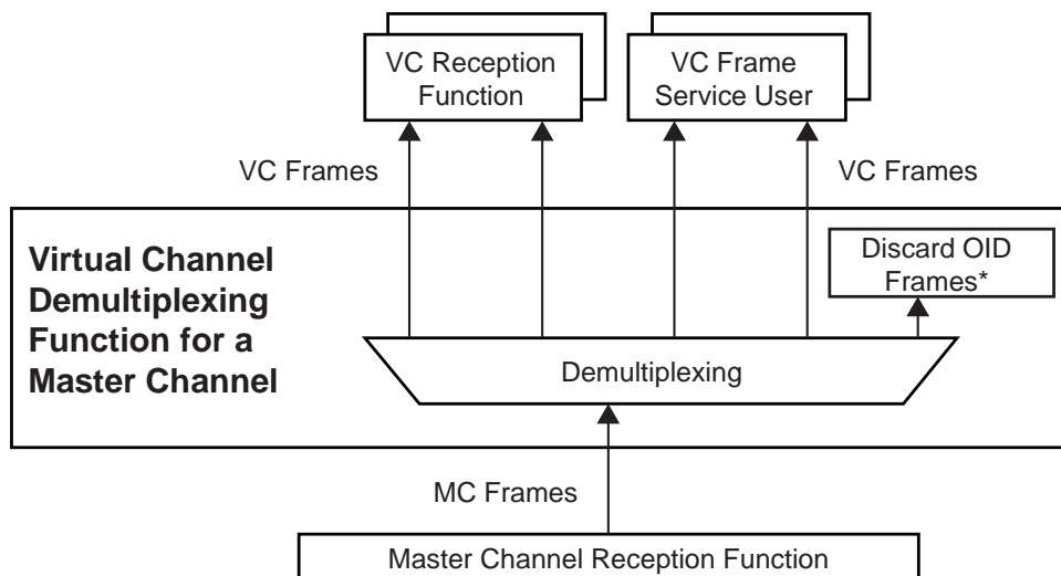
Figure 4-26: Abstract Model of Virtual Channel Demultiplexing Function
