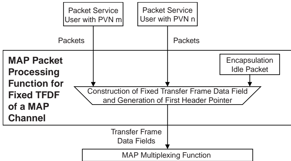
Figure 4-7: Abstract Model of Packet Processing Function for Fixed TFDFs
