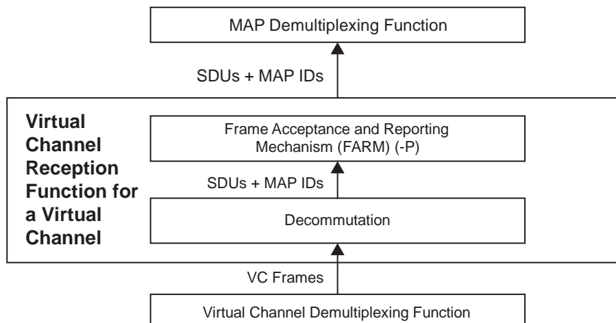
Figure 4-25: Abstract Model of Virtual Channel Reception Function
