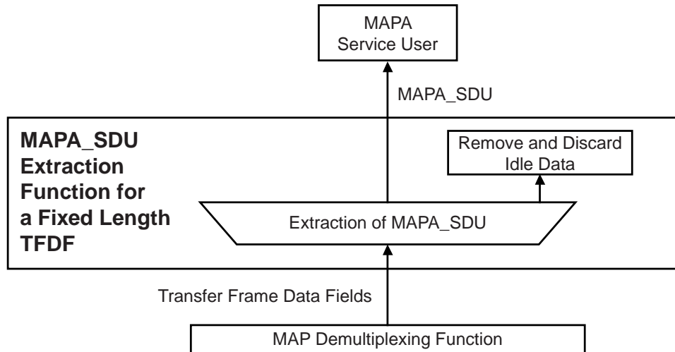
Figure 4-21: Abstract Model of MAPA_SDU Extraction Function for Fixed-Length TFDFs
