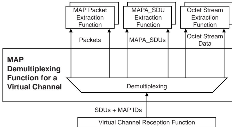
Figure 4-24: Abstract Model of MAP Demultiplexing Function
