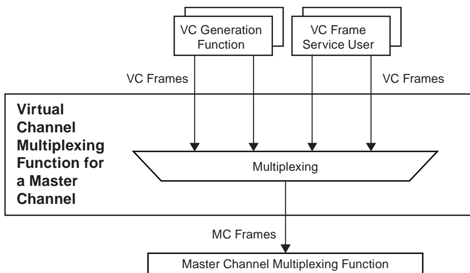
Figure 4-14: Abstract Model of Virtual Channel Multiplexing Function
