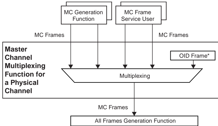
Figure 4-16: Abstract Model of Master Channel Multiplexing Function
