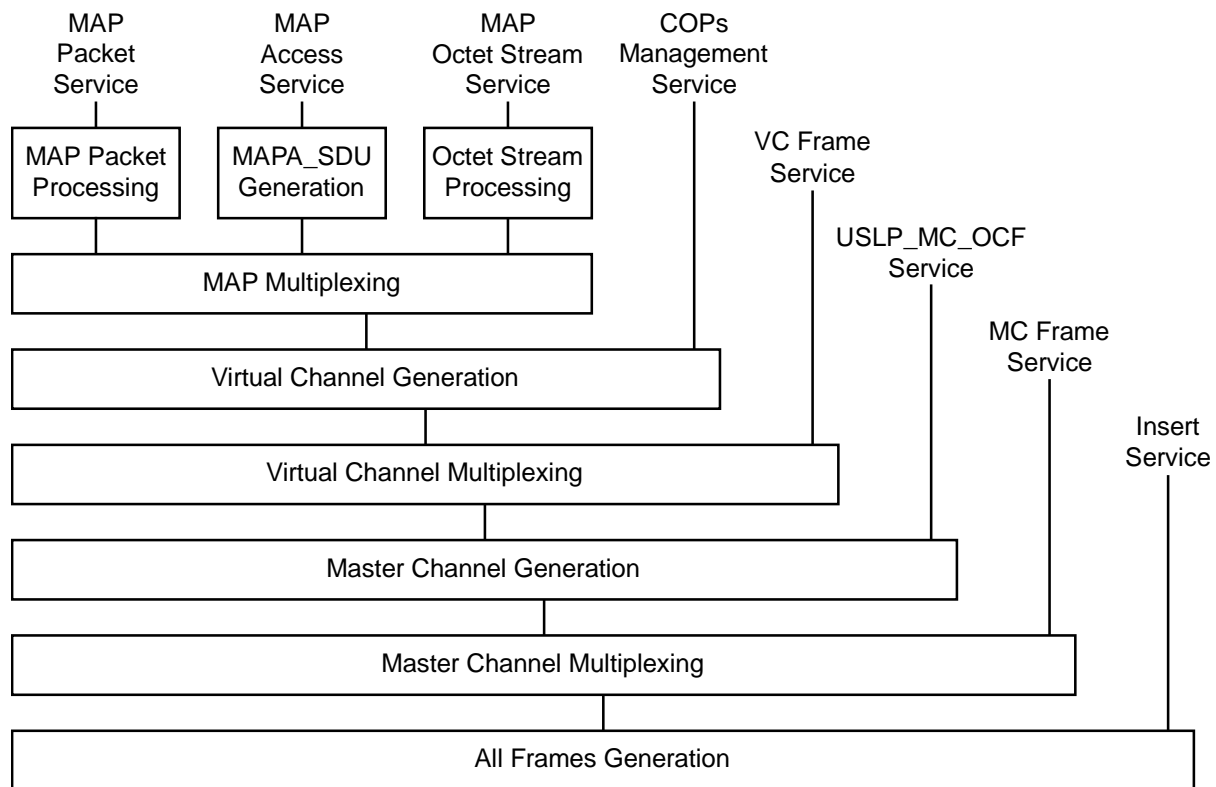
Figure 4-6: Internal Organization of Protocol Entity (Sending End)
