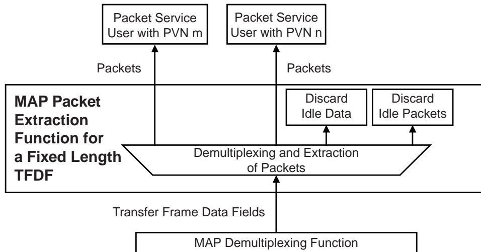
Figure 4-19: Abstract Model of MAP Packet Extraction Function for Fixed-Length TFDFs
