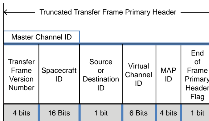
Figure 4-3: Truncated Transfer Frame Primary Header
