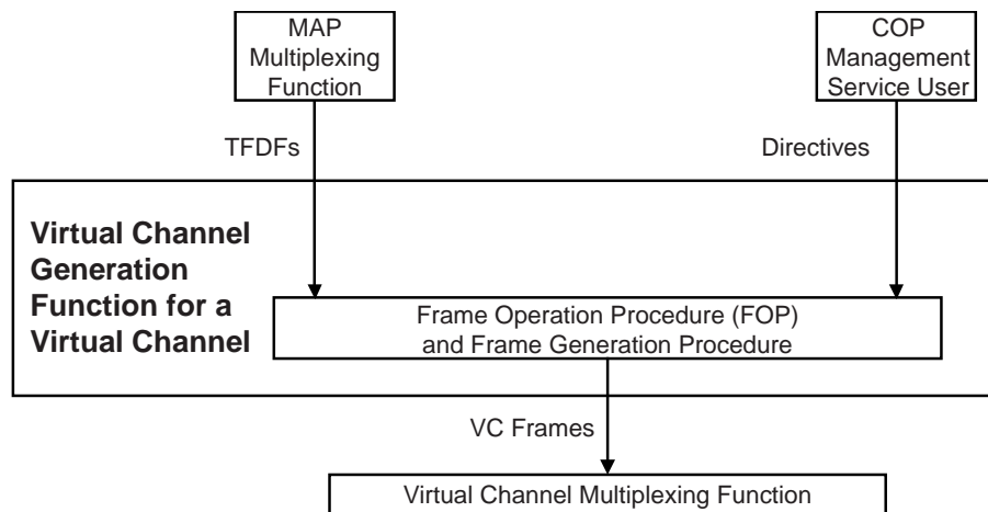
Figure 4-13: Abstract Model of Virtual Channel Generation Function
