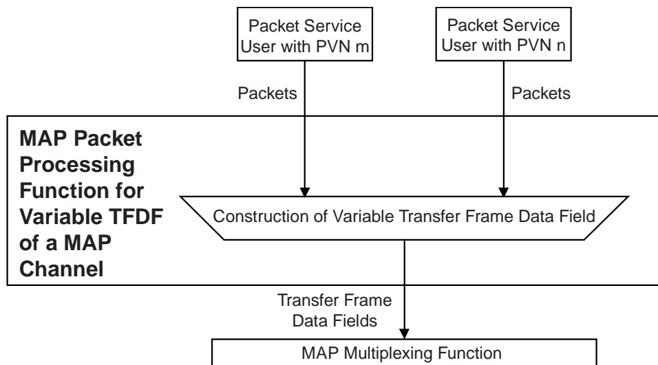
Figure 4-8: Abstract Model of MAP Packet Processing Function for Variable-Length TFDFs
