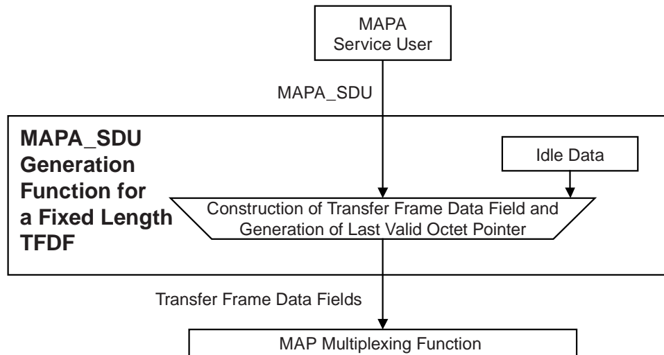
Figure 4-9: Abstract Model of MAPA_SDU Generation Function for Fixed-Length TFDFs
