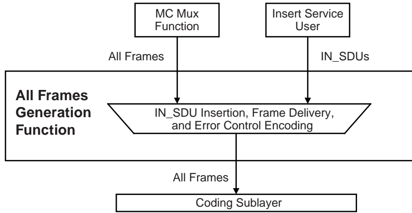
Figure 4-17: Abstract Model of All Frames Generation Function
