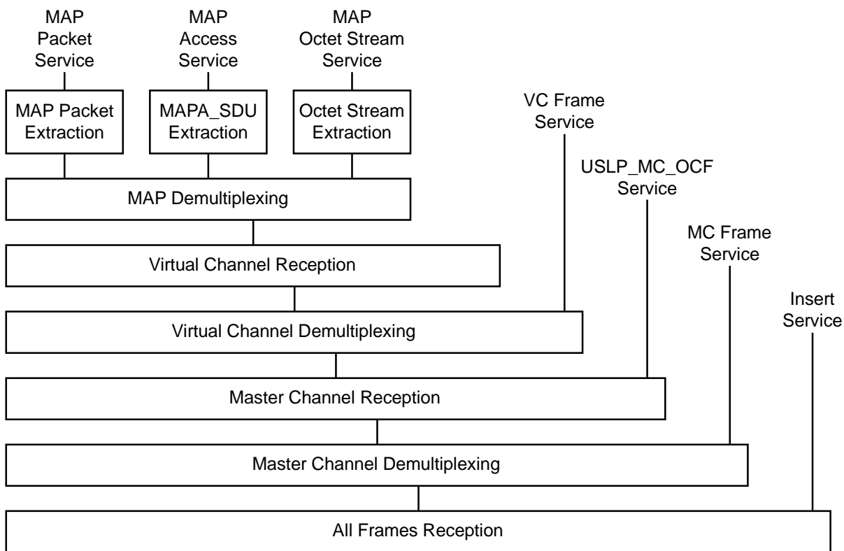
Figure 4-18: Internal Organization of Protocol Entity (Receiving End)
