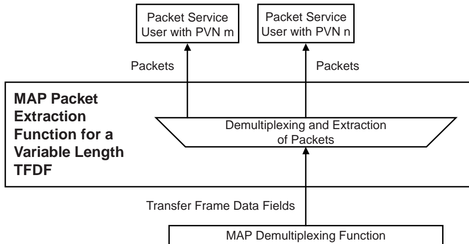
Figure 4-20: Abstract Model of MAP Packet Extraction Function for Variable-Length TFDs
