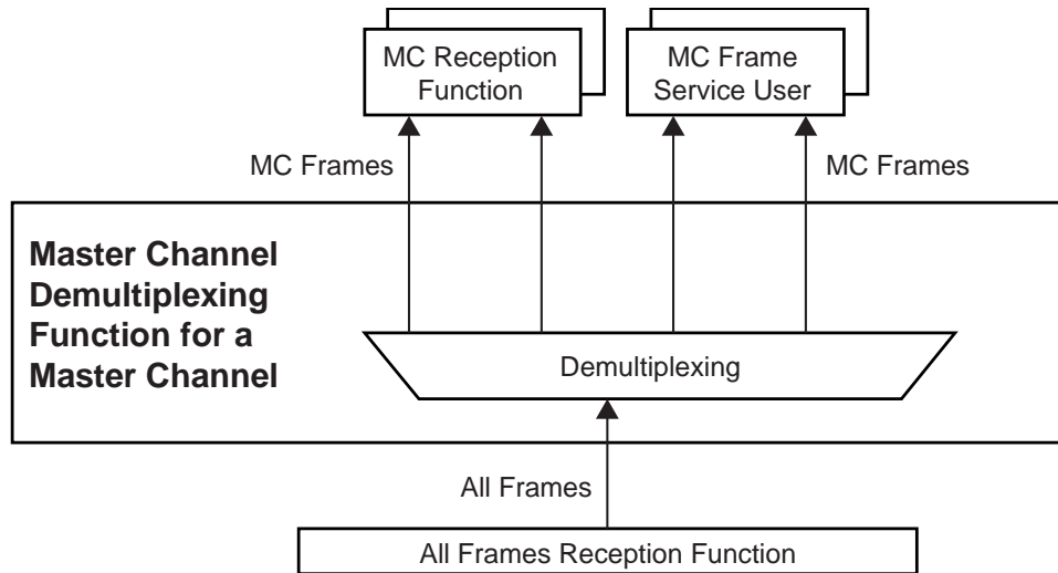
Figure 4-28: Abstract Model of Master Channel Demultiplexing Function
