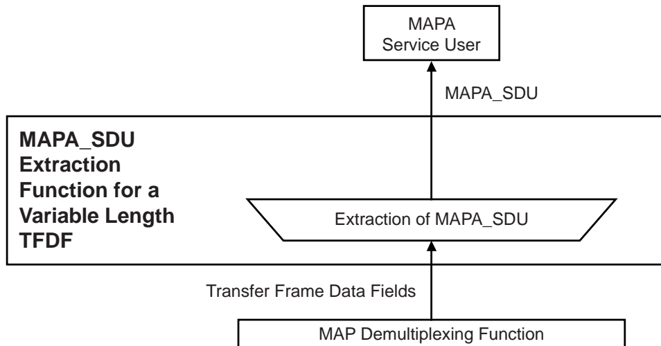
Figure 4-22: Abstract Model of MAPA_SDU Extraction Function for Variable-Length TFDs
