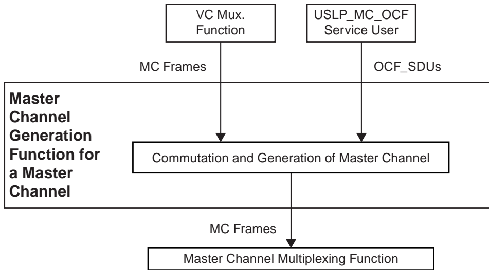
Figure 4-15: Abstract Model of the Master Channel Generation Function
