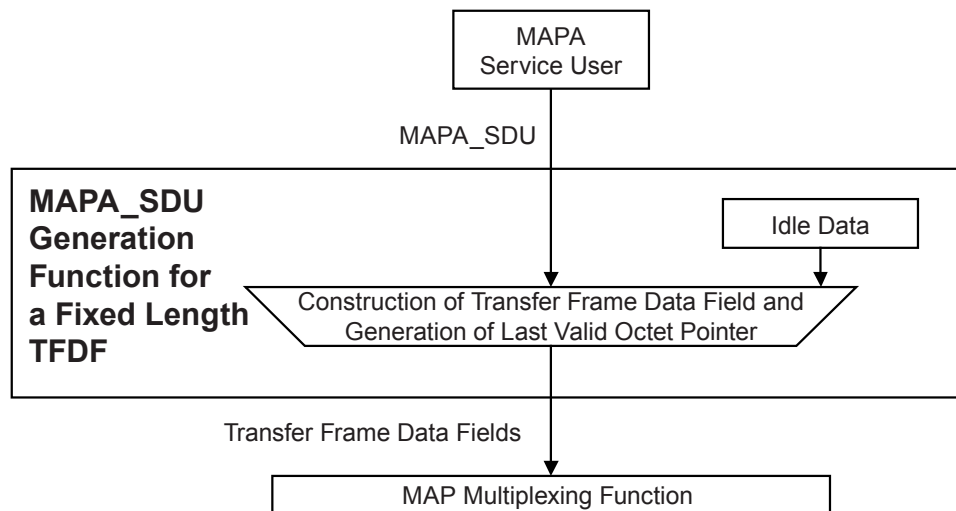
Figure 4-8: Abstract Model of MAPA_SDU Generation Function for Fixed-Length TFDFs
