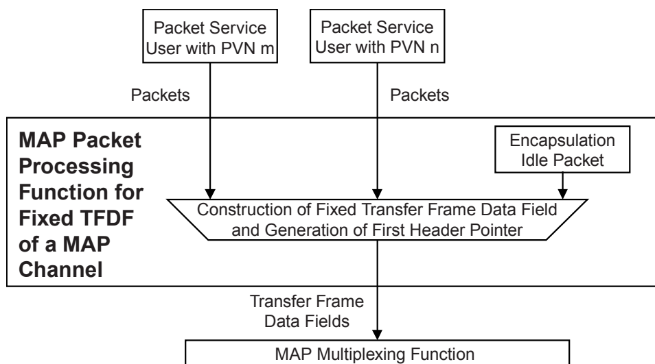
Figure 4-6: Abstract Model of Packet Processing Function for Fixed TFDs
