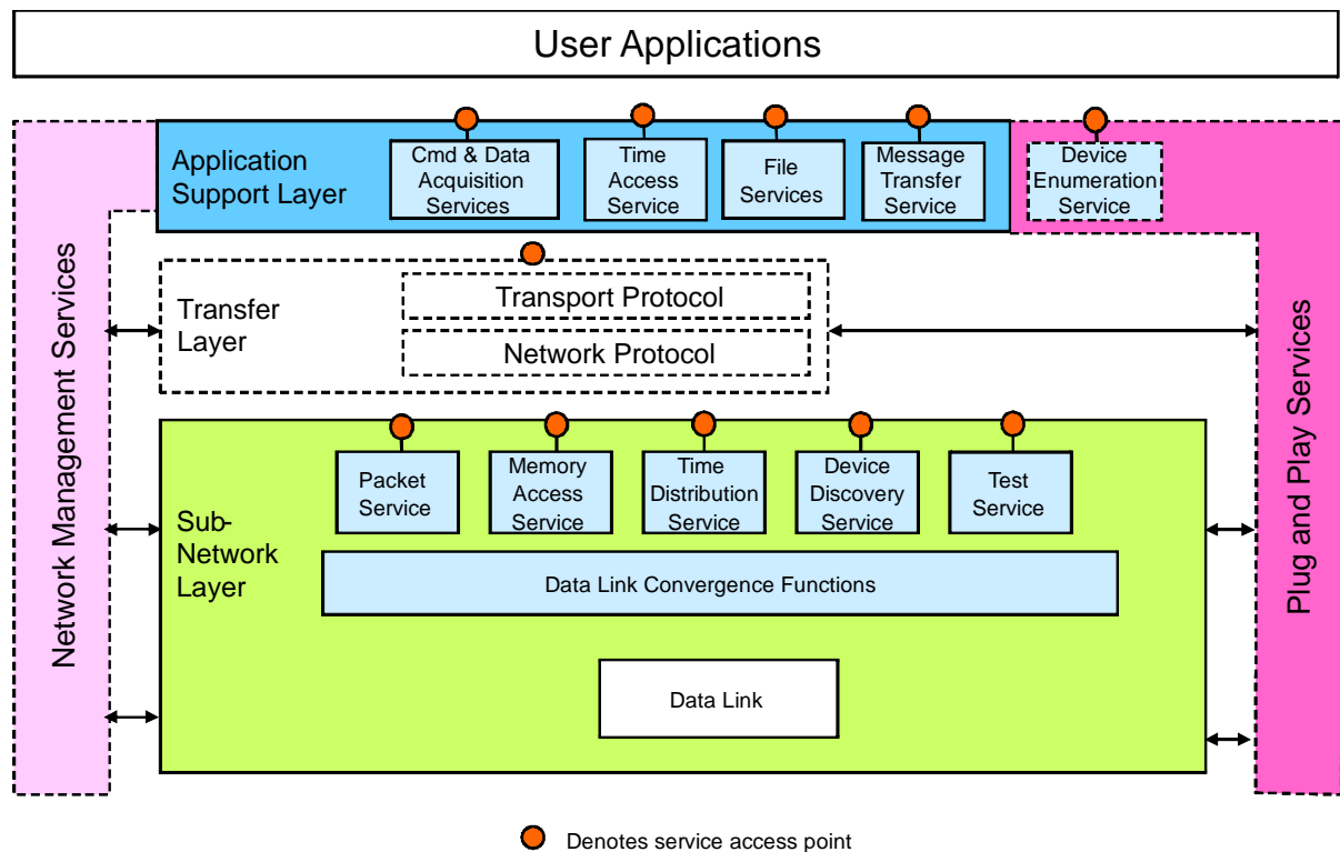
Figure 2-1: SOIS Architecture
