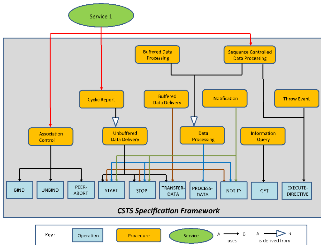
Figure 2-2: CSTS Directly Composed of CSTS Specification Framework Procedures
