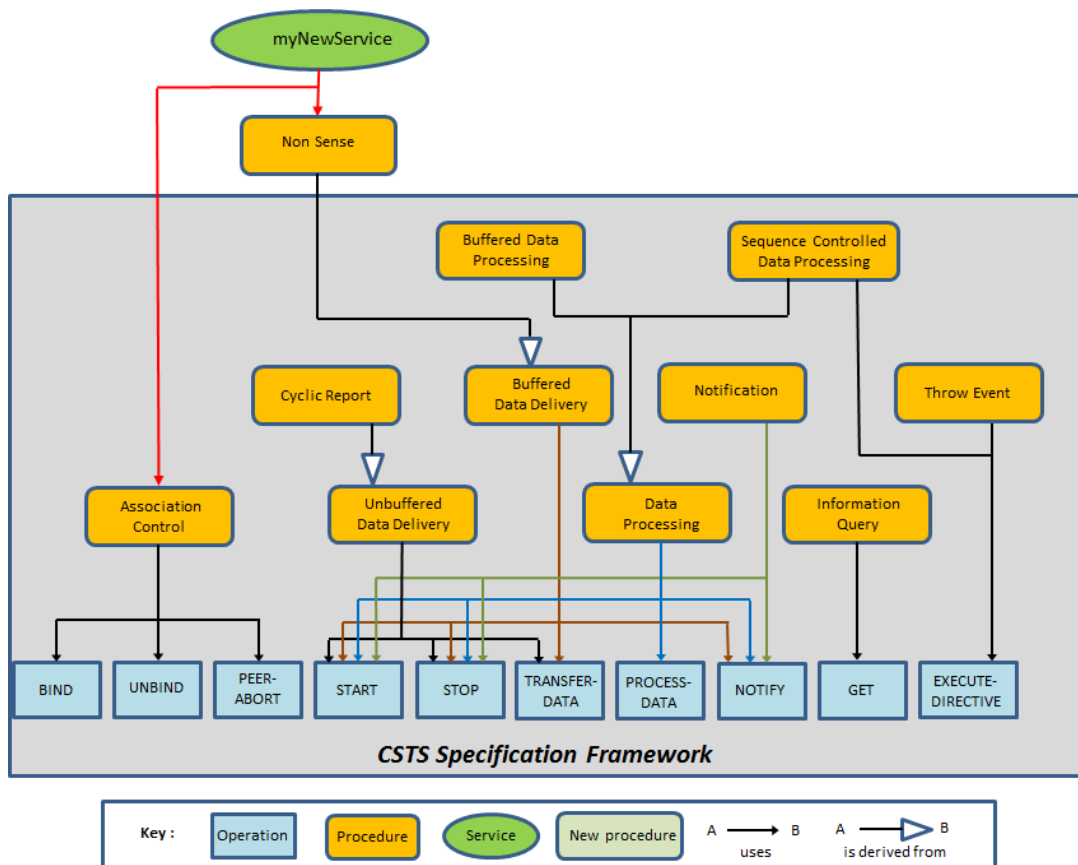
Figure C-1: MyNewService CSTS Composition and Derivation
