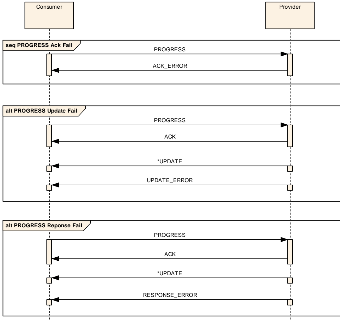
Figure 3-16: PROGRESS Interaction Pattern Error Sequence
