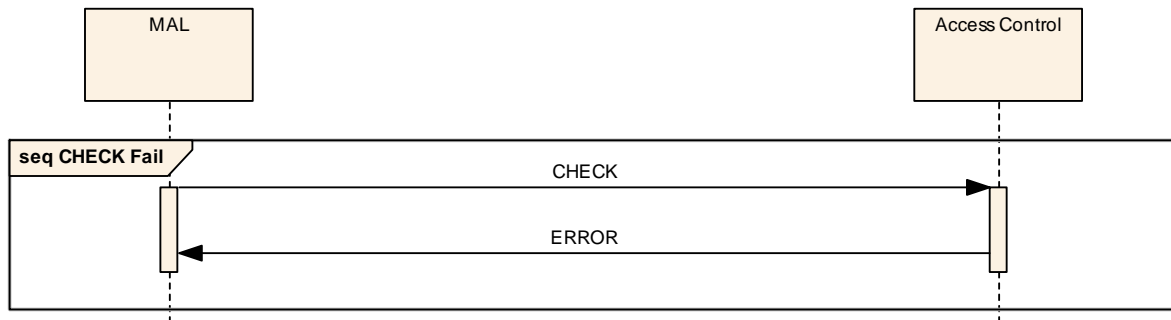
Figure 3-28: CHECK Access Control Pattern Error Sequence
