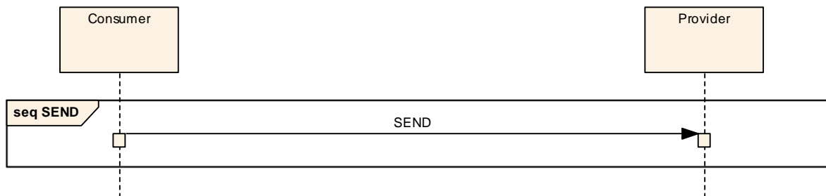
Figure 3-2: SEND Interaction Pattern Message Sequence
