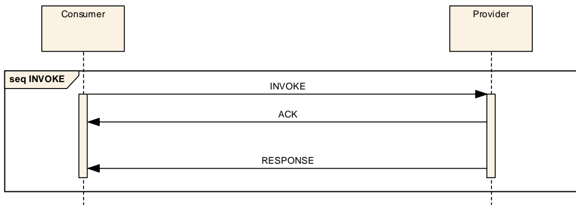
Figure 3-11: INVOKE Interaction Pattern Message Sequence
