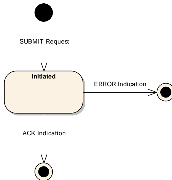
Figure 3-5: SUBMIT Consumer State Chart
