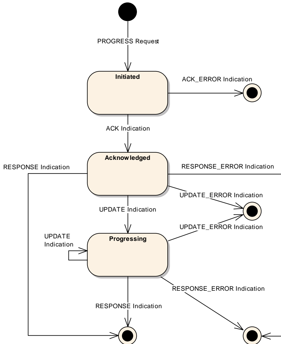
Figure 3-17: PROGRESS Consumer State Chart
