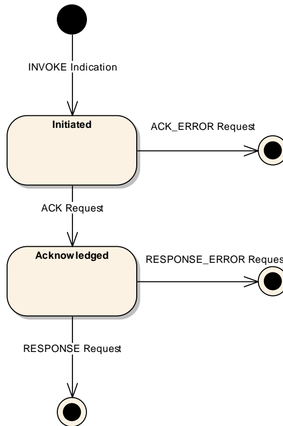
Figure 3-14: INVOKE Provider State Chart
