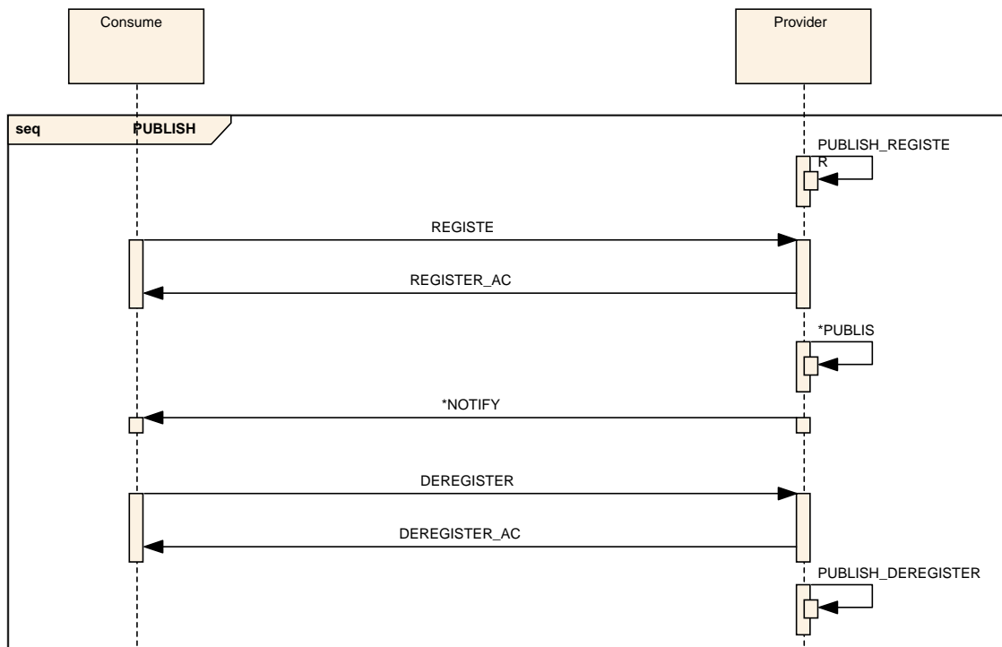
Figure 3-20: PUBLISH-SUBSCRIBE Pattern Alternative Message Sequence
