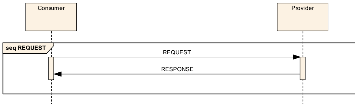
Figure 3-7: REQUEST Interaction Pattern Message Sequence
