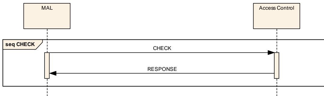
Figure 3-27: CHECK Access Control Pattern Message Sequence
