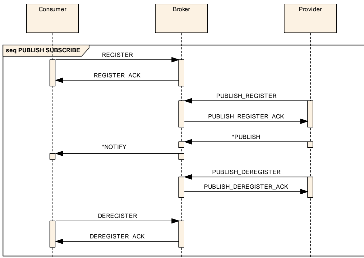
Figure 3-19: PUBLISH-SUBSCRIBE Interaction Pattern Message Sequence
