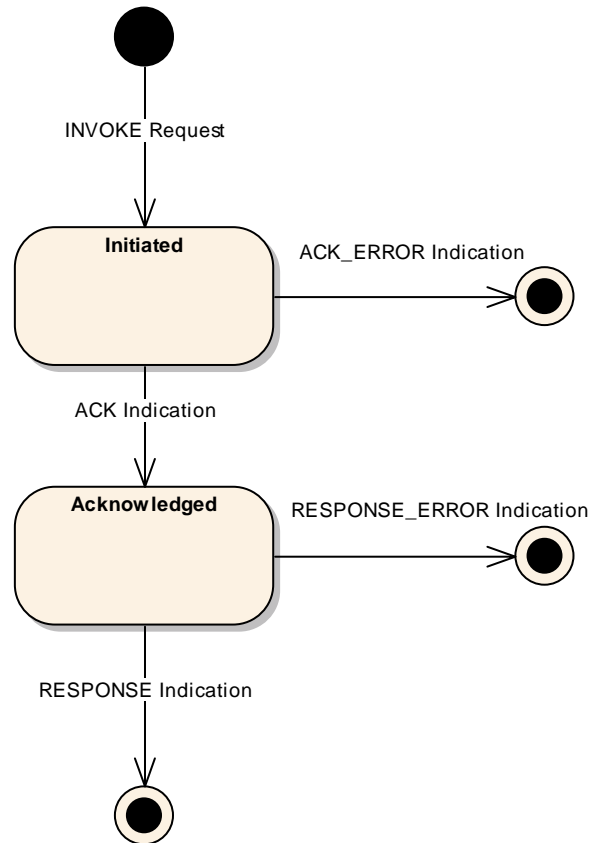
Figure 3-13: INVOKE Consumer State Chart
