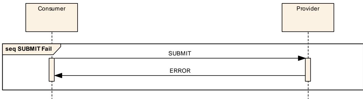
Figure 3-4: SUBMIT Interaction Pattern Error Sequence
