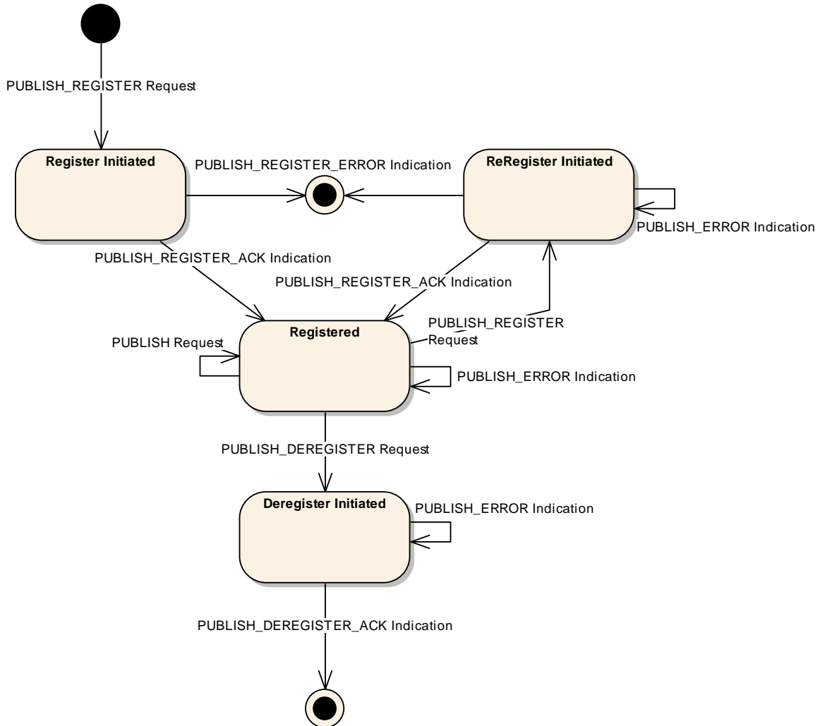
Figure 3-25: PUBLISH-SUBSCRIBE Provider State Chart
