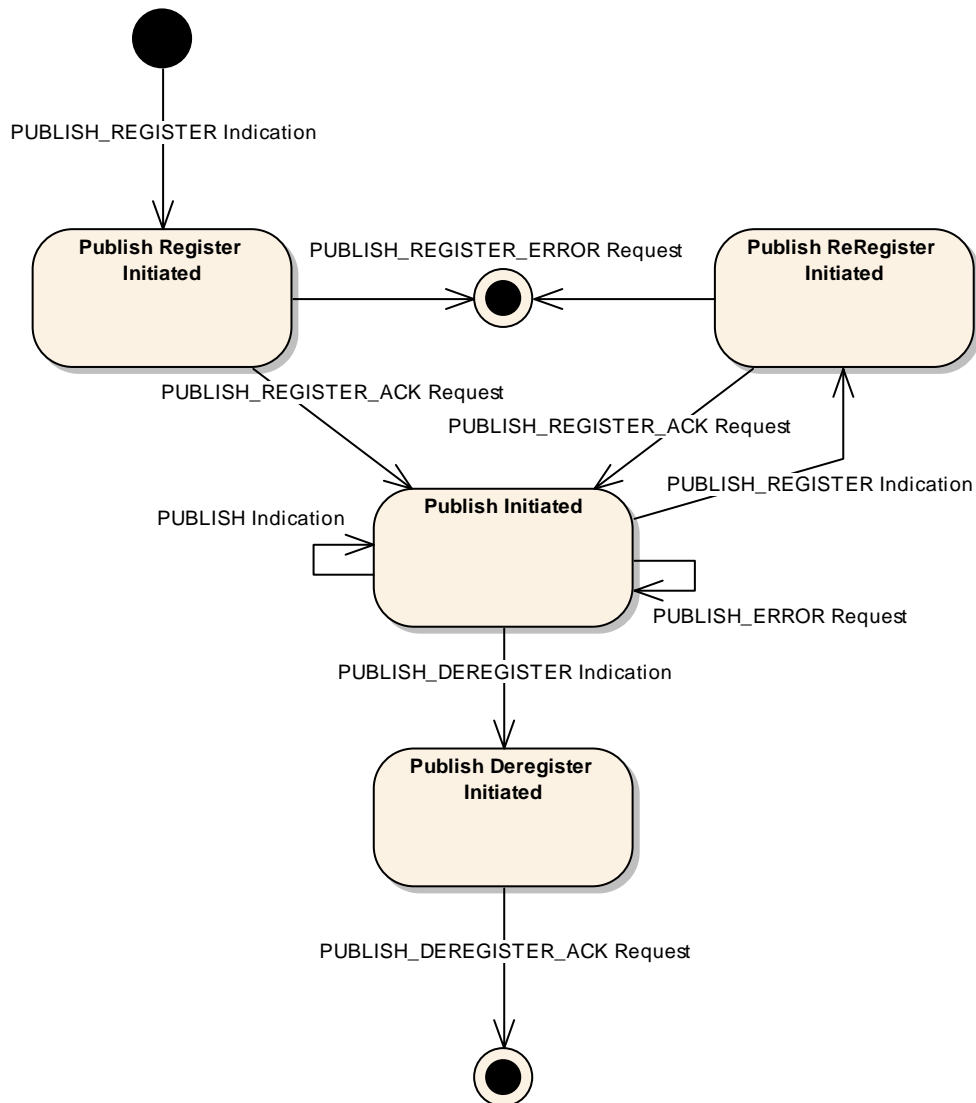
Figure 3-26: PUBLISH-SUBSCRIBE Broker to Provider State Chart
