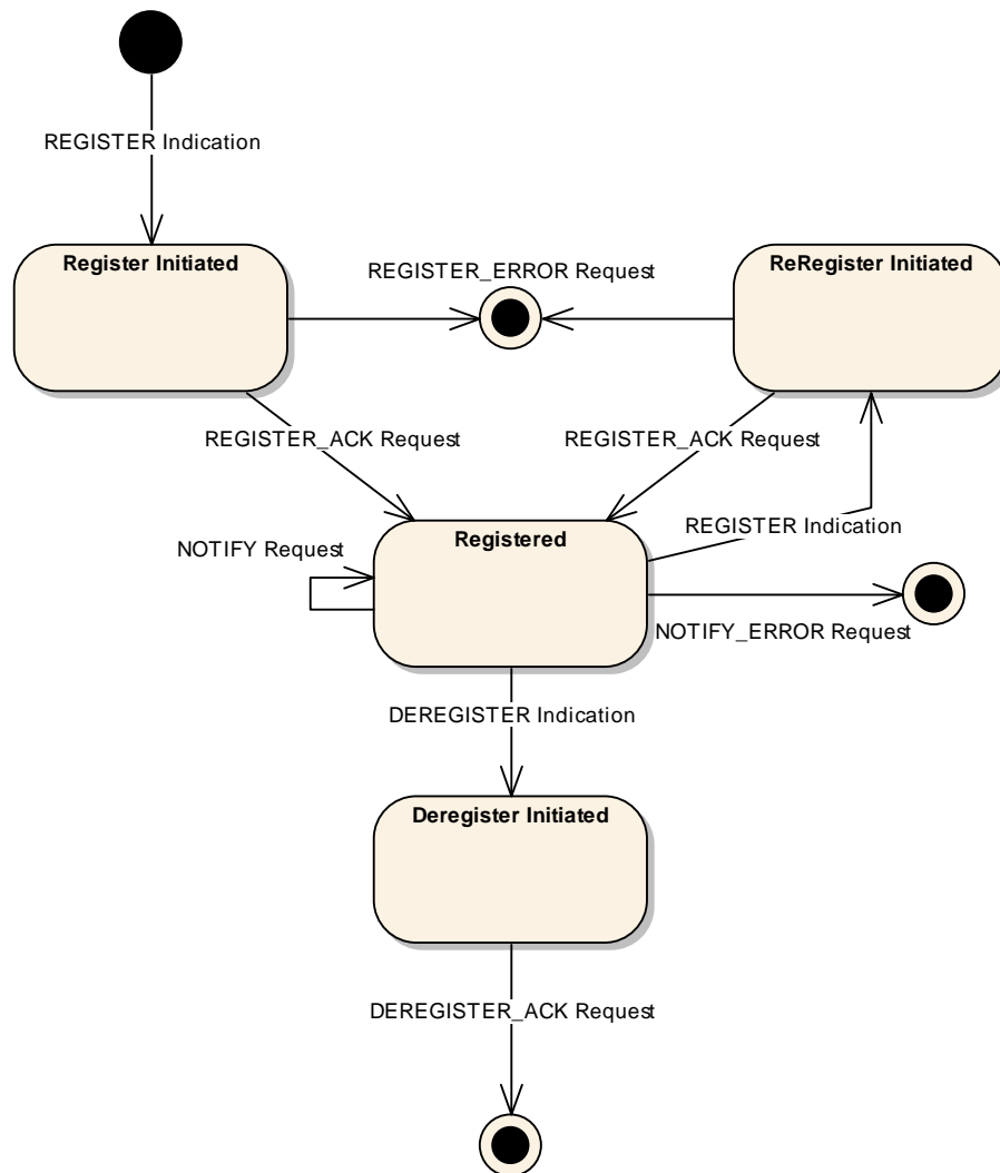
Figure 3-24: PUBLISH-SUBSCRIBE Broker to Consumer State Chart
