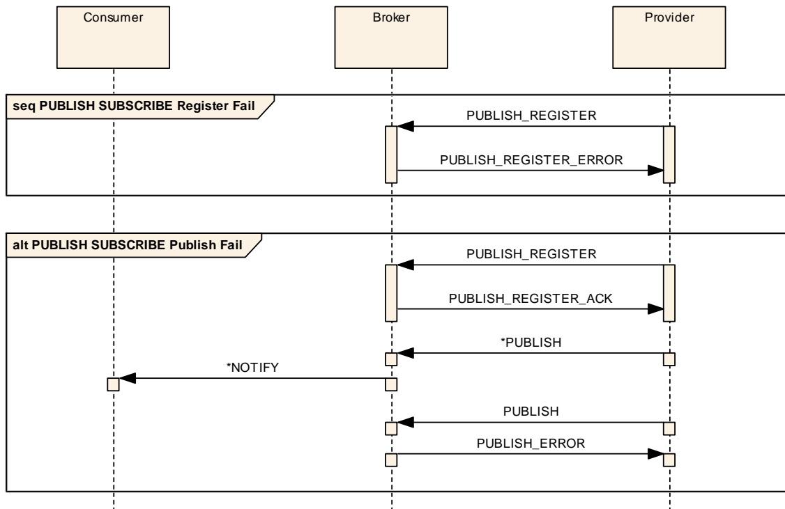
Figure 3-22: PUBLISH-SUBSCRIBE Interaction Pattern Provider Error Sequence
