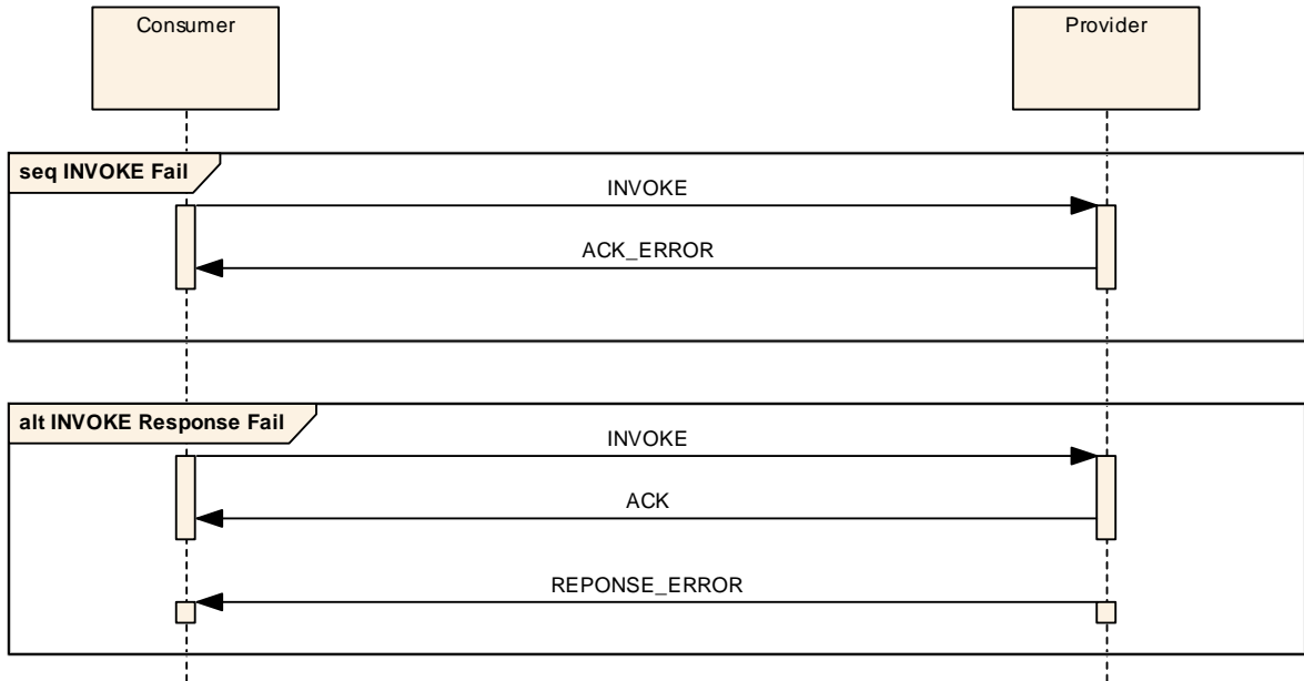
Figure 3-12: INVOKE Interaction Pattern Error Sequence
