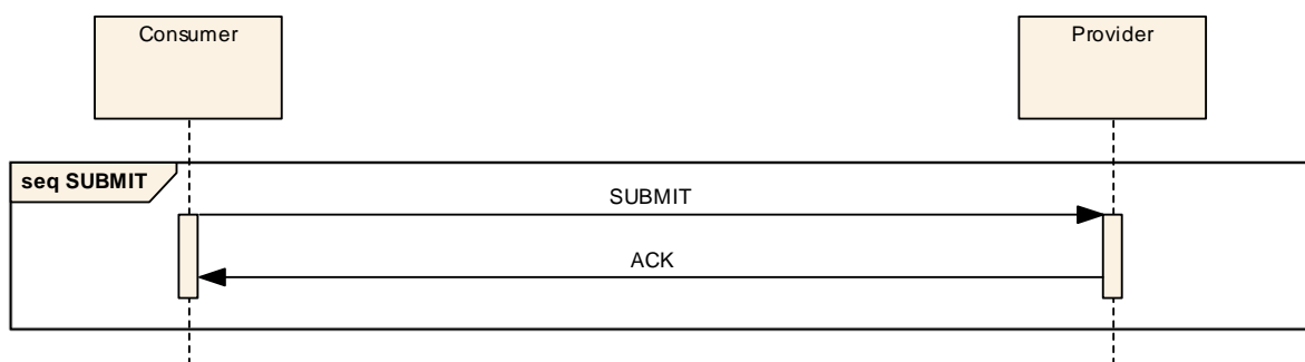
Figure 3-3: SUBMIT Interaction Pattern Message Sequence
