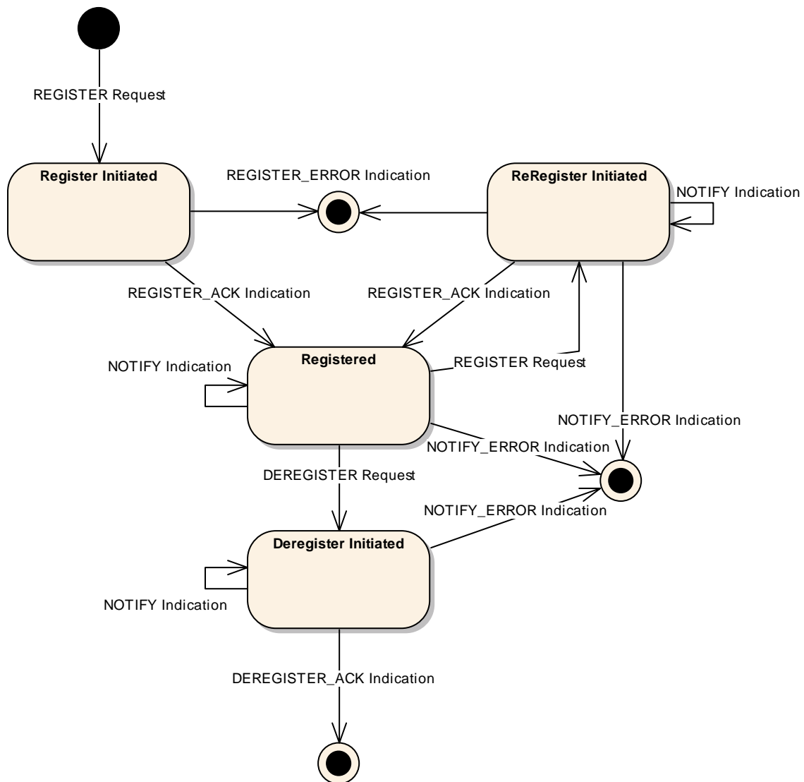
Figure 3-23: PUBLISH-SUBSCRIBE Consumer State Chart
