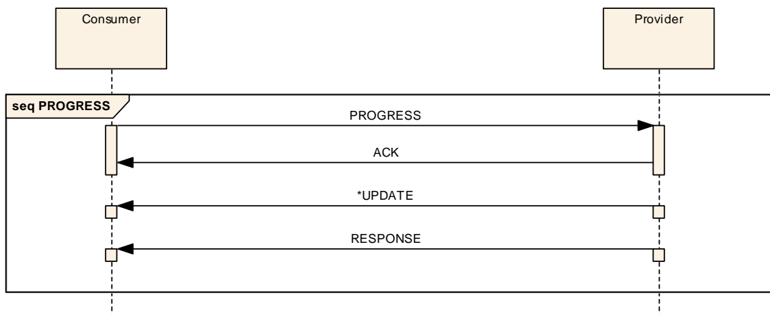
Figure 3-15: PROGRESS Interaction Pattern Message Sequence
