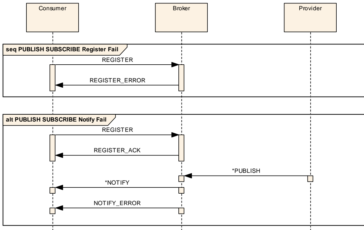
Figure 3-21: PUBLISH-SUBSCRIBE Interaction Pattern Consumer Error Sequence
