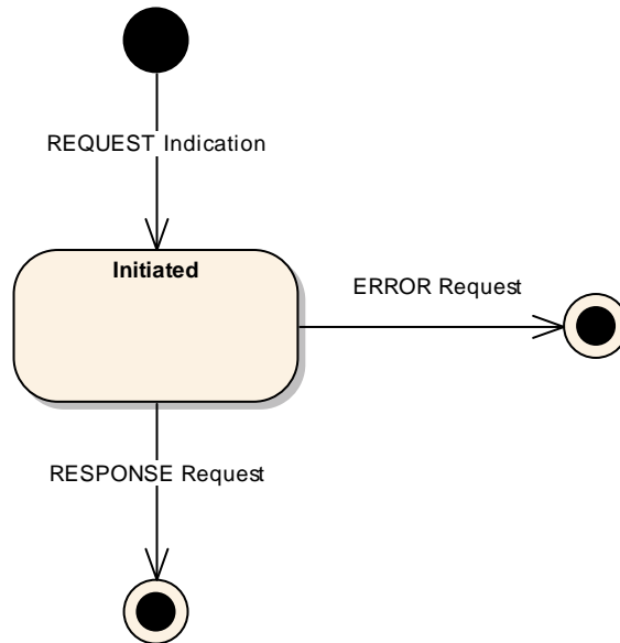
Figure 3-10: REQUEST Provider State Chart
