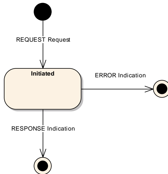
Figure 3-9: REQUEST Consumer State Chart
