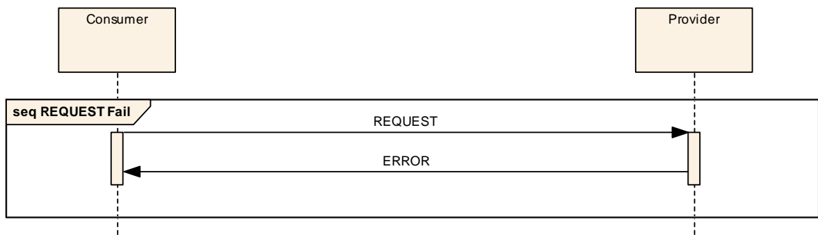
Figure 3-8: REQUEST Interaction Pattern Error Sequence
