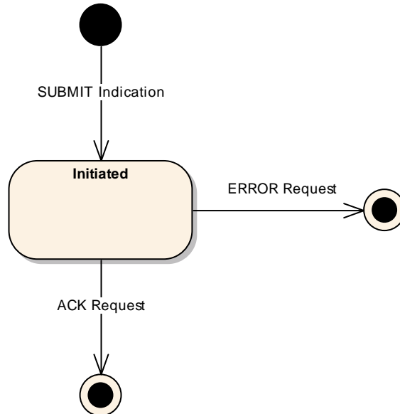
Figure 3-6: SUBMIT Provider State Chart
