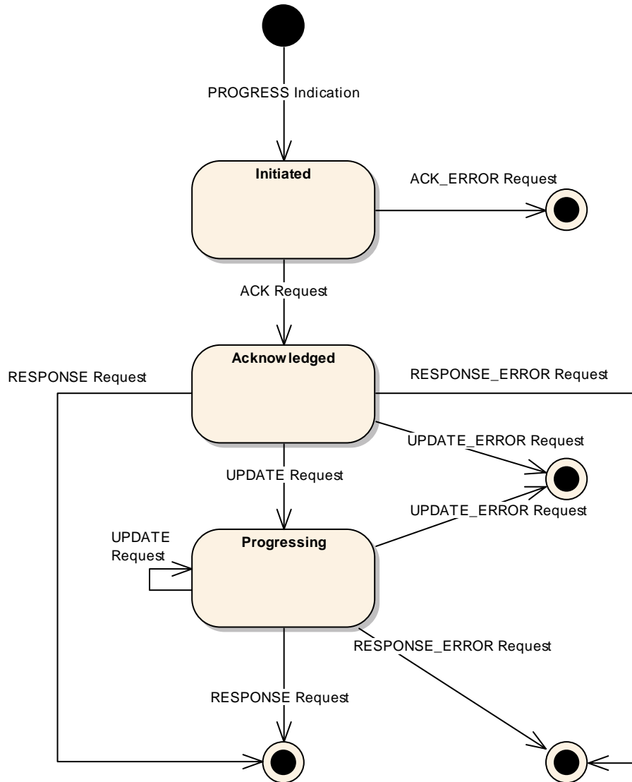
Figure 3-18: PROGRESS Provider State Chart
