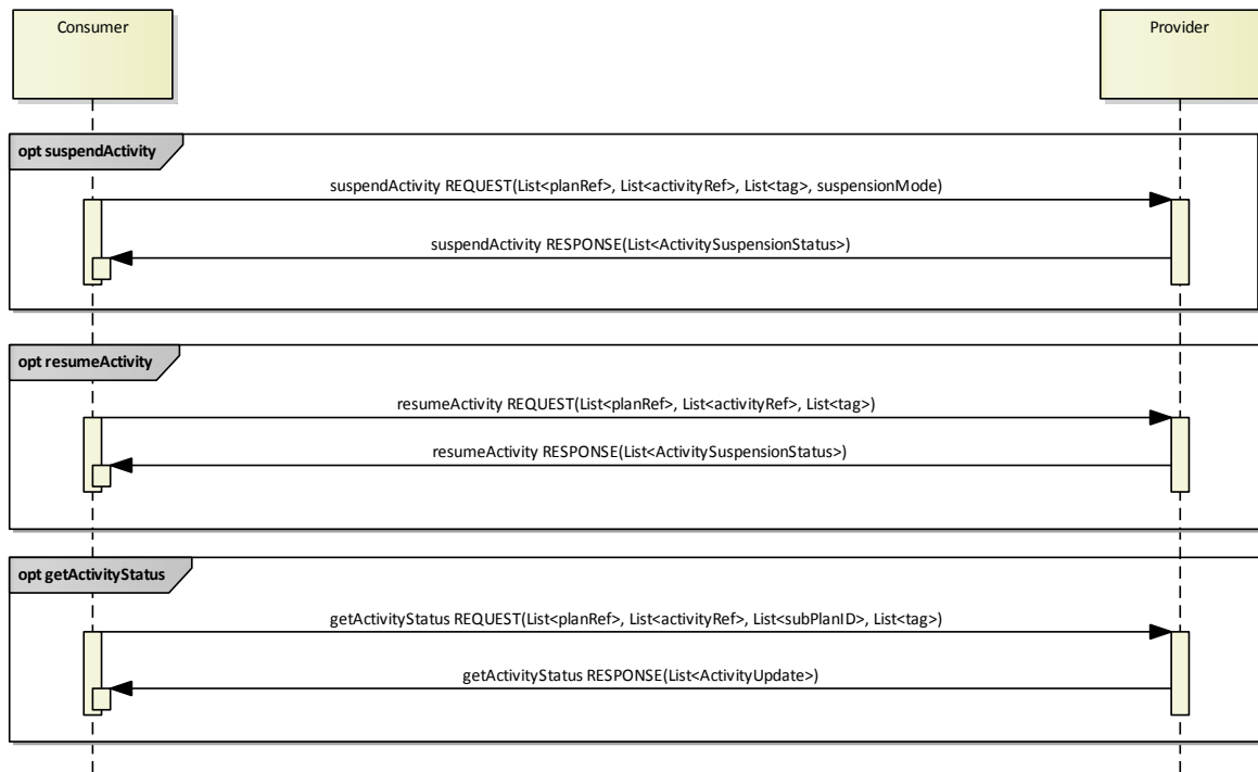
Figure 3-9: Activity Execution Control Operations
