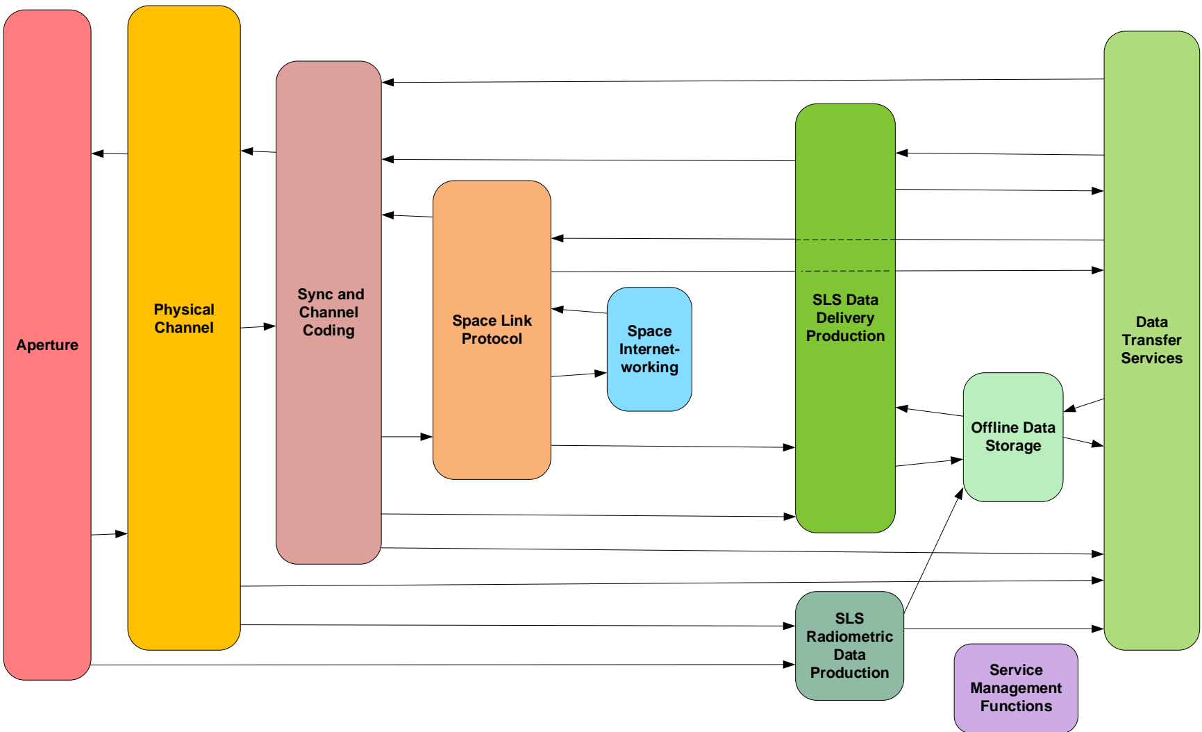
Figure 2-2: Functional Resource Strata for Earth-Space Link Terminals
