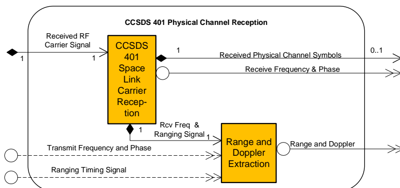
Figure 4-2: Member Functional Resources of the CCSDS 401 Physical Channel Reception Functional Resource Set
