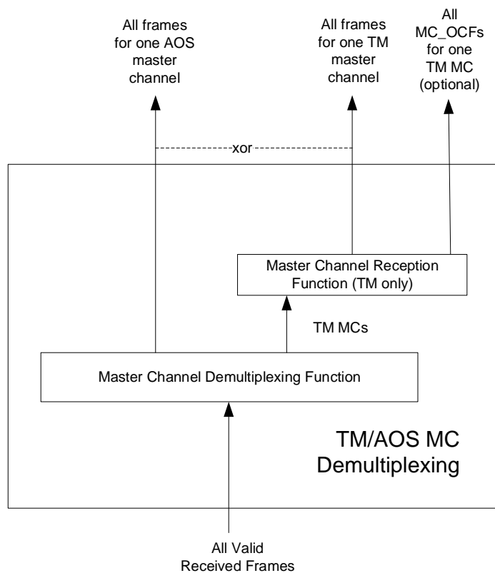
Figure 6-10: Internal Structure of the TM/AOS MC Demultiplexing Functional Resource
