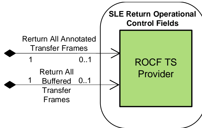
Figure 10-5: Member Functional Resource of the Return Operational Control Fields Functional Resource Set
