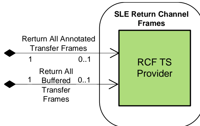
Figure 10-4: Member Functional Resource of the Return Channel Frames Functional Resource Set
