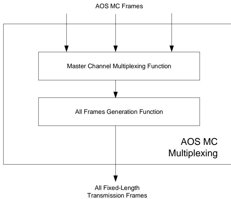
Figure 6-4: Internal Structure of the AOS MC Multiplexing Functional Resource
