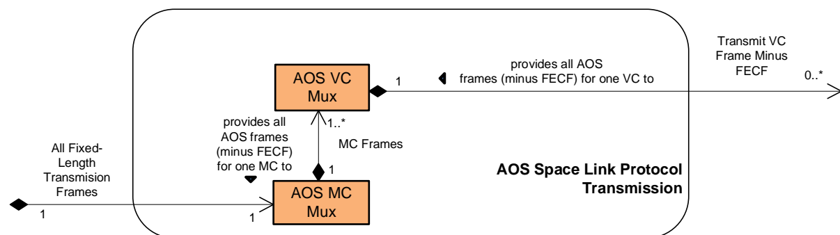
Figure 6-3: Members of the AOS Space Link Protocol Transmission Functional Resource Set
