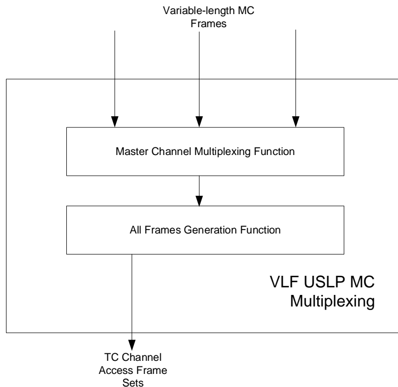
Figure 6-6: Internal Structure of the VLF USLP MC Multiplexing Functional Resource
