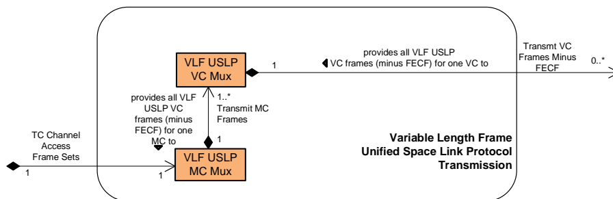
Figure 6-5: Member Functional Resources of the VLF Unified Space Link Protocol Transmission Functional Resource Set
