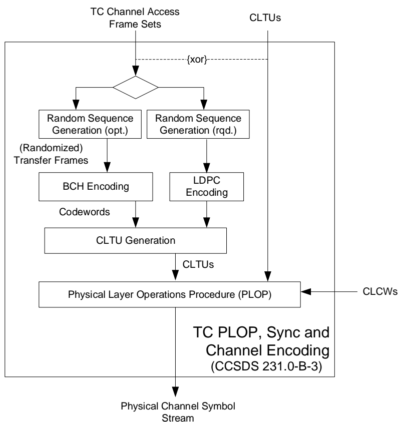
Figure 5-2: Internal Structure of the TC PLOP, Synchronization and Channel Encoding Functional Resource Corresponding to CCSDS 231.0-B-3
