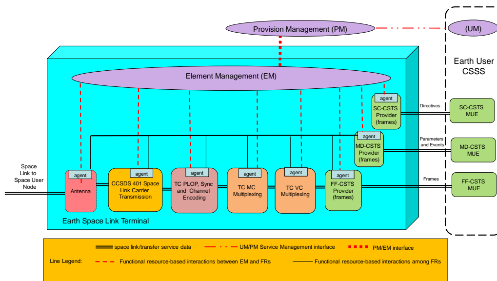
Figure 2-7: Functional Resource Conceptual Model of Interaction
