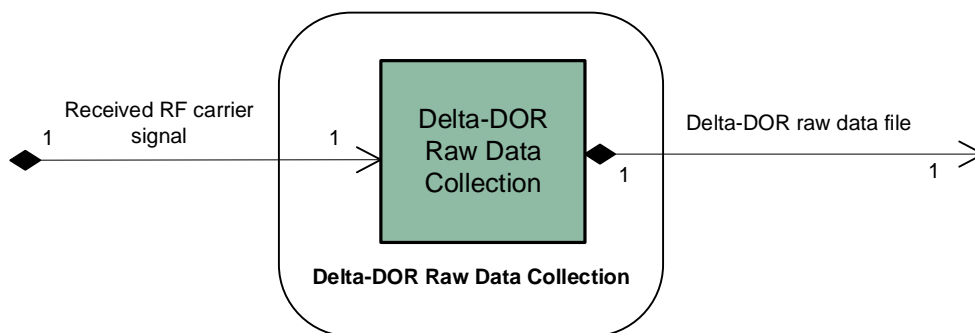
Figure 4-3: Member Functional Resource of the Delta-DOR Raw Data Collection Functional Resource Set
