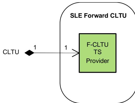
Figure 10-1: Member Functional Resource of the SLE Forward CLTU Functional Resource Set
