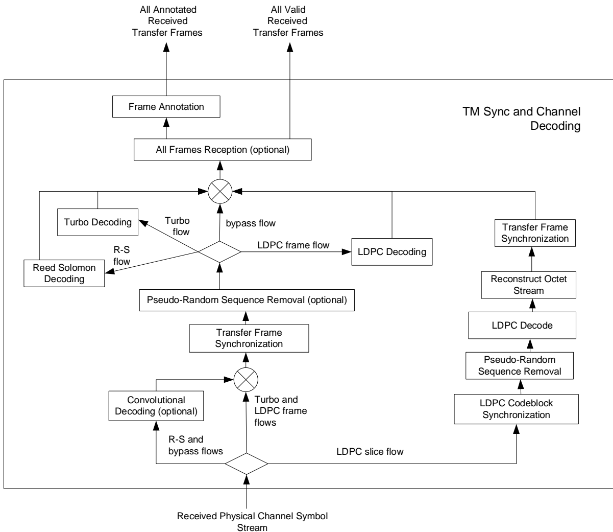
Figure 5-7: Internal Structure of the TM Synchronization and Channel Decoding Functional Resource
