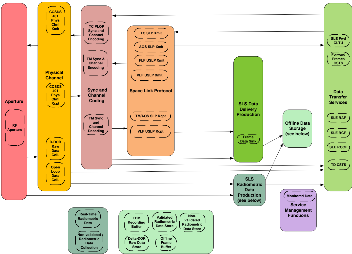
Figure 2-4: Functional Resource Strata Used in SLS Configurations
