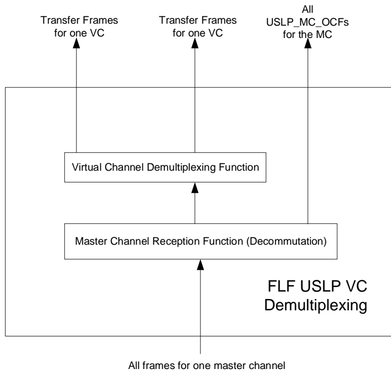
Figure 6-13: Internal Structure of the FLF USLP VC Demultiplexing FR
