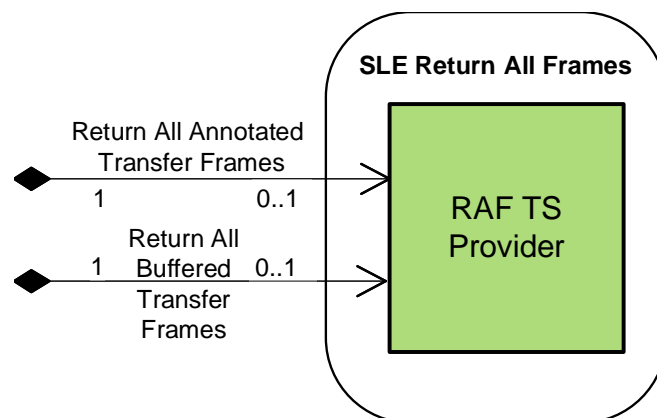
Figure 10-3: Member Functional Resource of the Return All Frames Functional Resource Set
