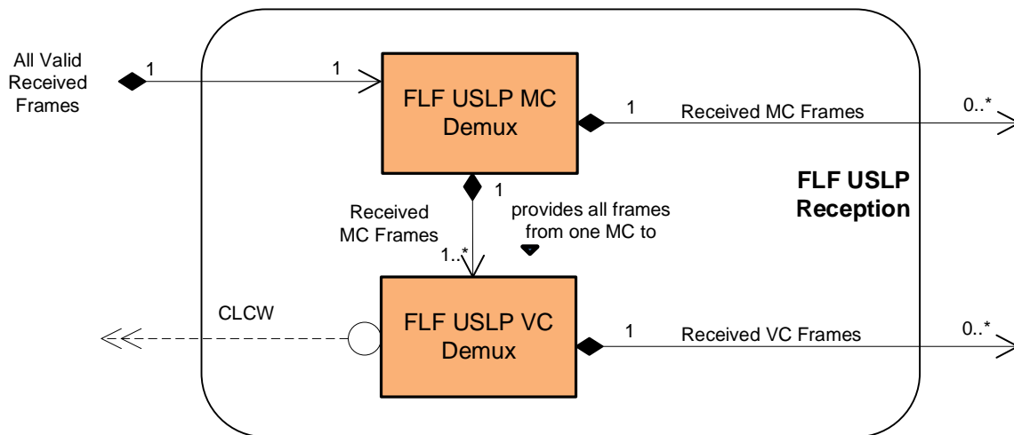
Figure 6-12: Member Functional Resources of the FLF USLP Reception Functional Resource Set
