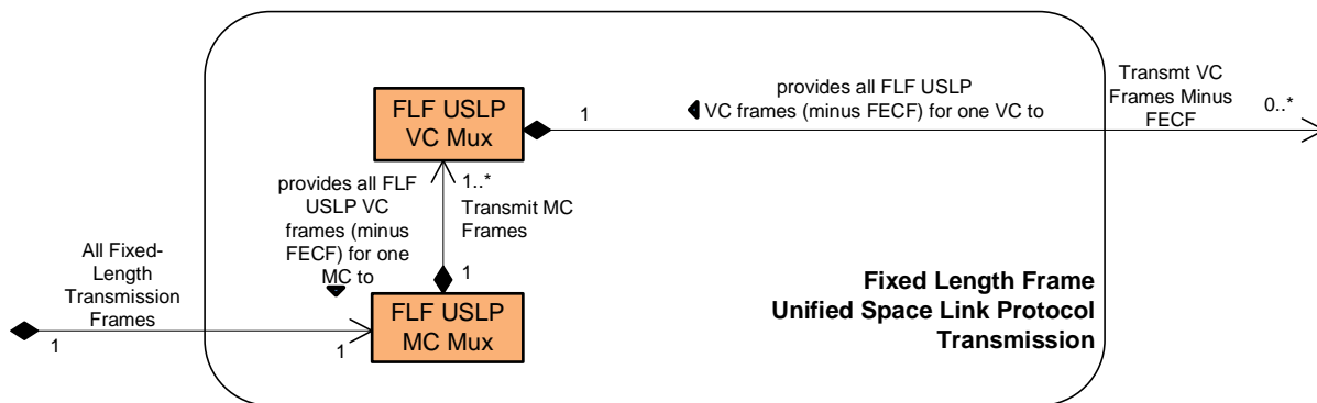
Figure 6-7: Member Functional Resources of the FLF Unified Space Link Protocol Transmission Functional Resource Set
