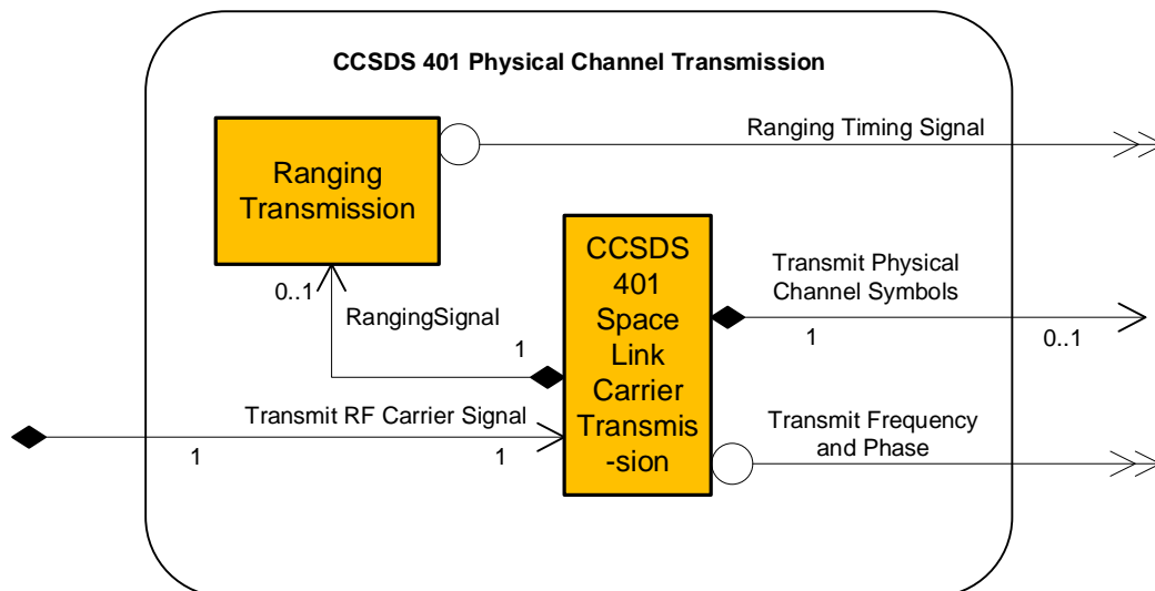
Figure 4-1: Member Functional Resources of the CCSDS 401 Physical Channel Transmission Functional Resource Set
