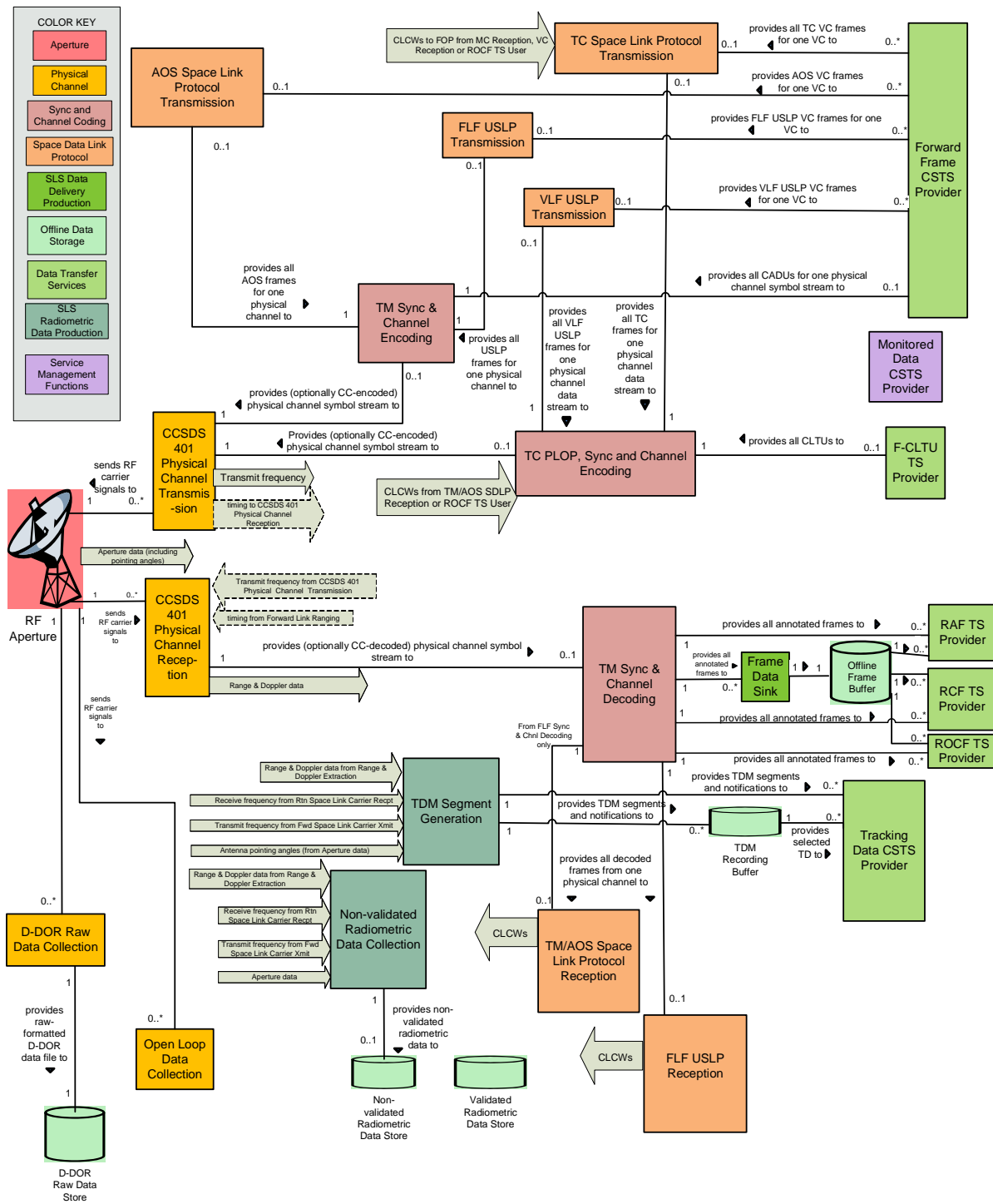
Figure 2-6: Functional Resource Set Connectivity
