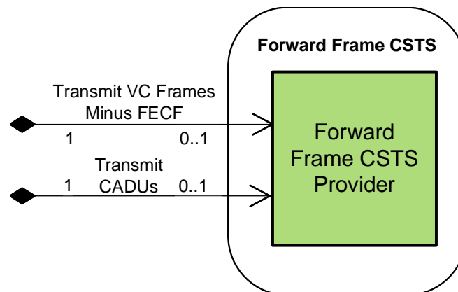
Figure 10-2: Member of the Forward Frame CSTS Functional Resource Set
