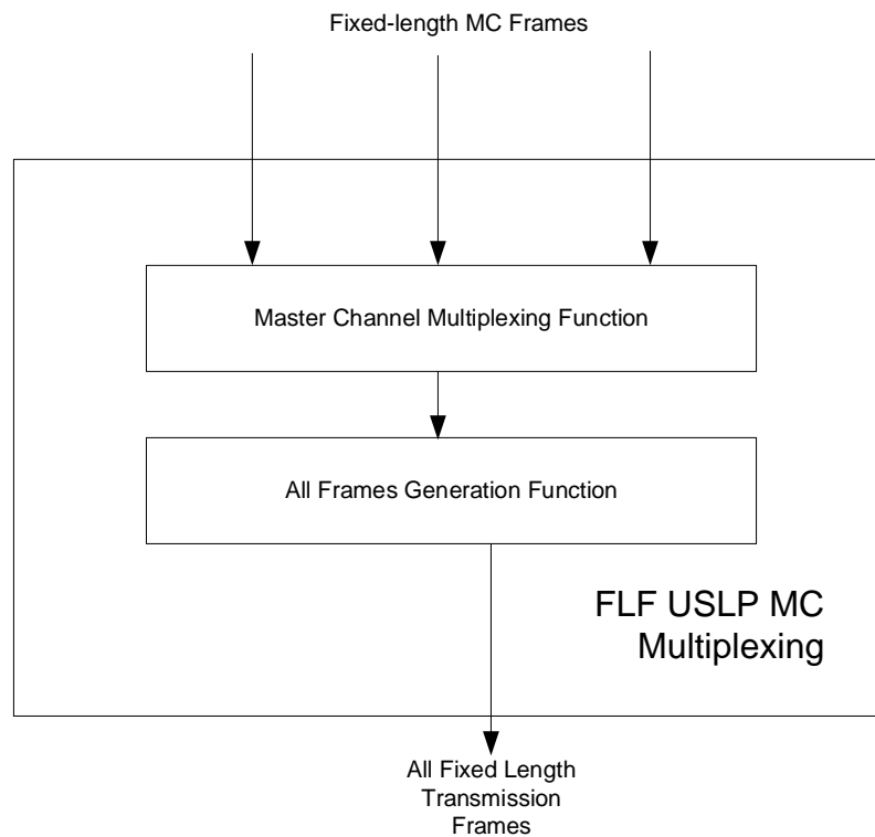
Figure 6-8: Internal Structure of the FLF USLP MC Multiplexing Functional Resource
