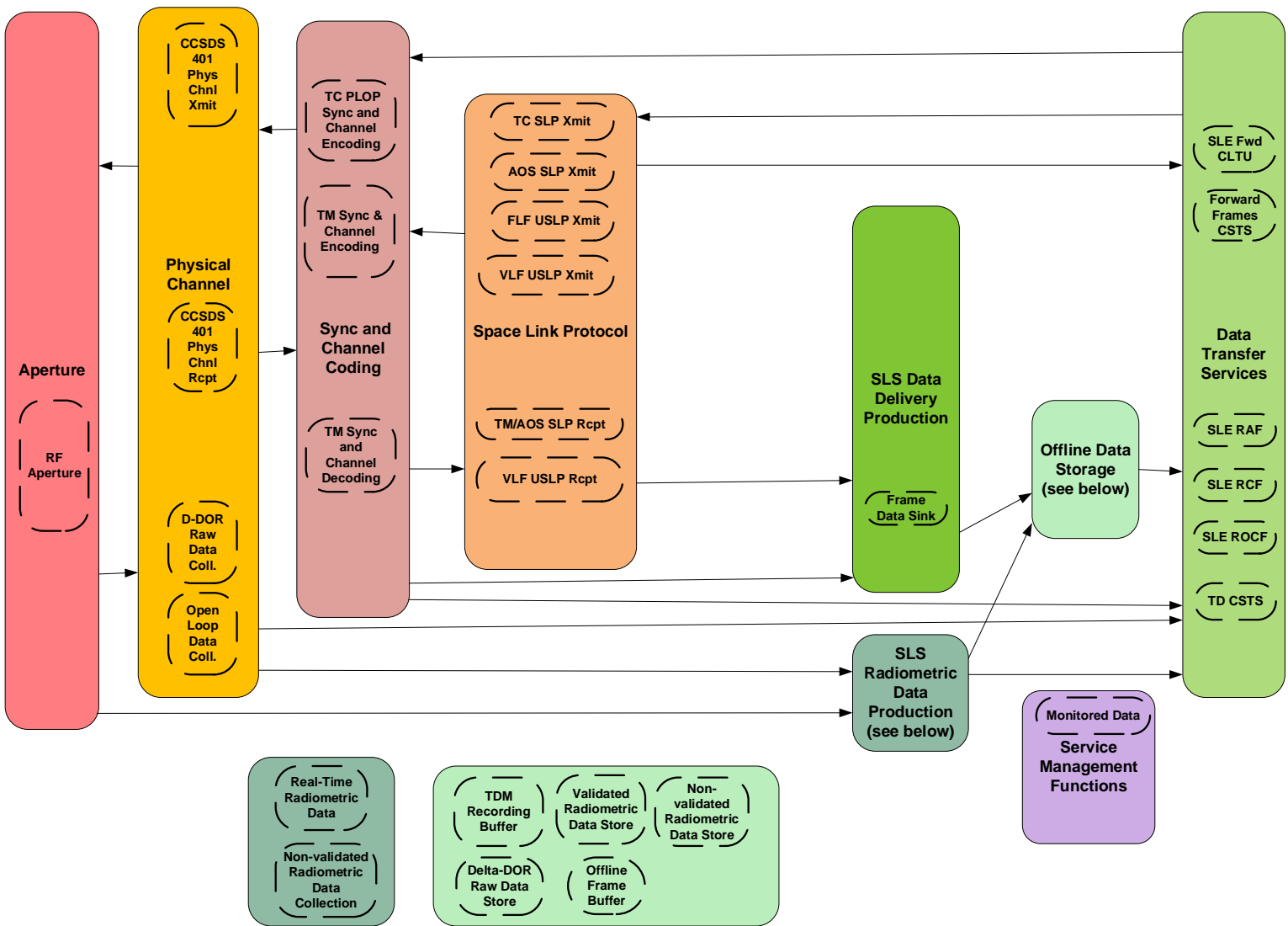
Figure 2-3: Functional Resources Sets within the Strata
