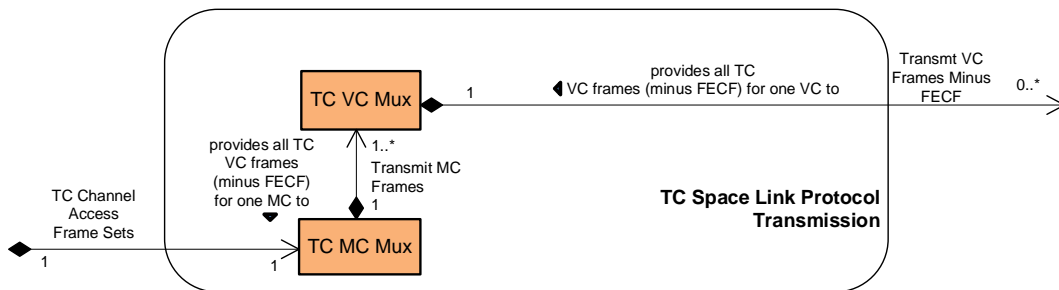
Figure 6-1: Member Functional Resources of the TC Space Link Protocol Transmission Functional Resource Set
