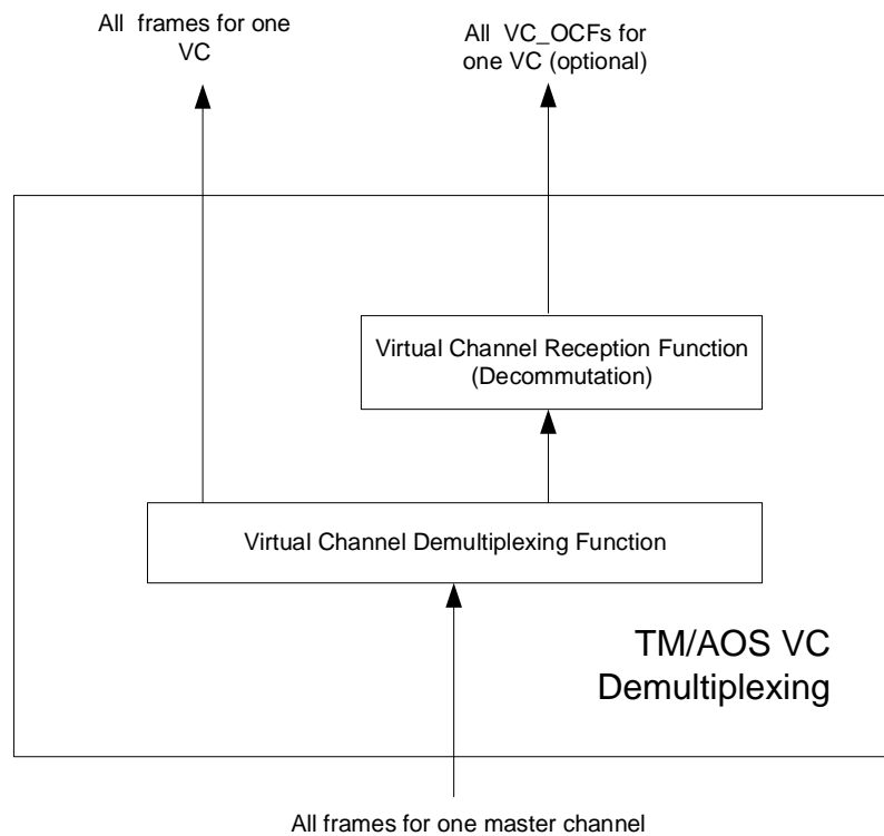
Figure 6-11: Internal Structure of the TM/AOS VC Demultiplexing FR
