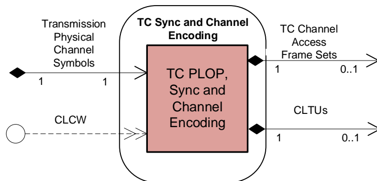
Figure 5-1: Member Functional Resource of the TC Synchronization and Channel Encoding Functional Resource Set
