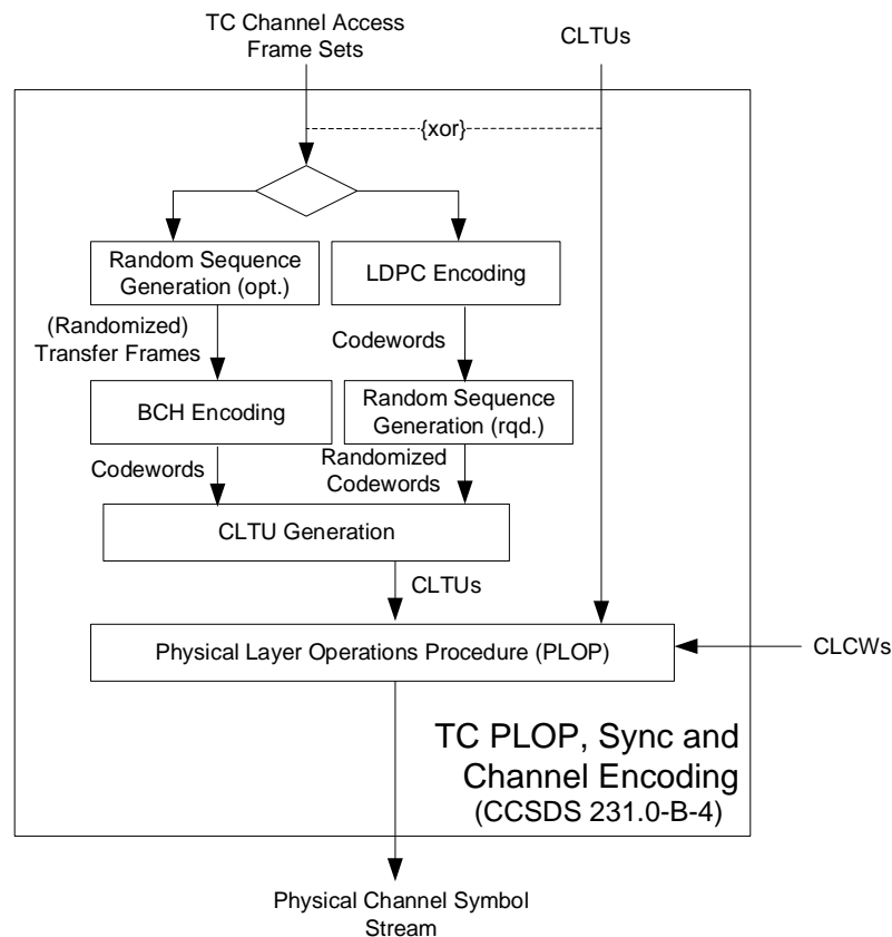
Figure 5-3: Internal Structure of the TC PLOP, Synchronization and Channel Encoding Functional Resource Corresponding to CCSDS 231.0-B-4
