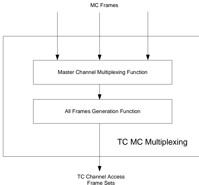
Figure 6-2: Internal Structure of the TC MC Multiplexing Functional Resource
