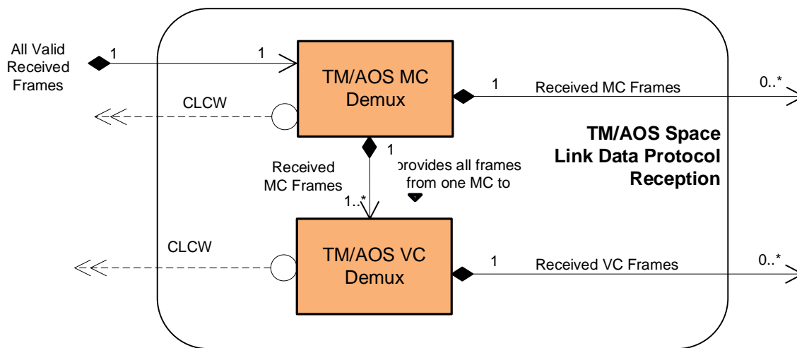
Figure 6-9: Member Functional Resources of the TM/AOS Space Link Protocol Reception Functional Resource Set
