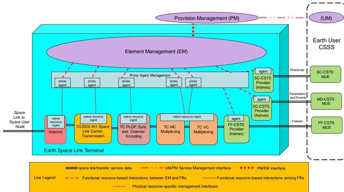
Figure 2-8: Functional Resource Mixed Architecture Example
