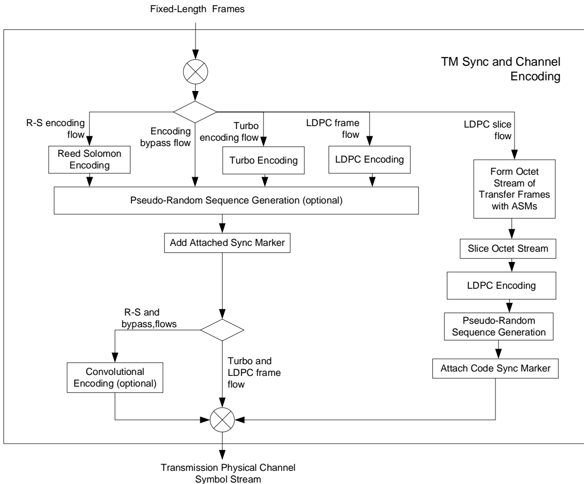
Figure 5-5: Internal Structure of the TM Synchronization and Channel Encoding Functional Resource
